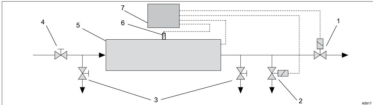
Fig. 1: Typical installation schematic of a UV system
