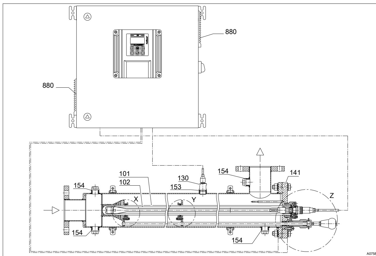
Fig. 53: Spare parts drawing Dulcodes R, spare parts list, see Chapter 10.2 'Spare parts list for UV-systems with manual wiper' on page 77
