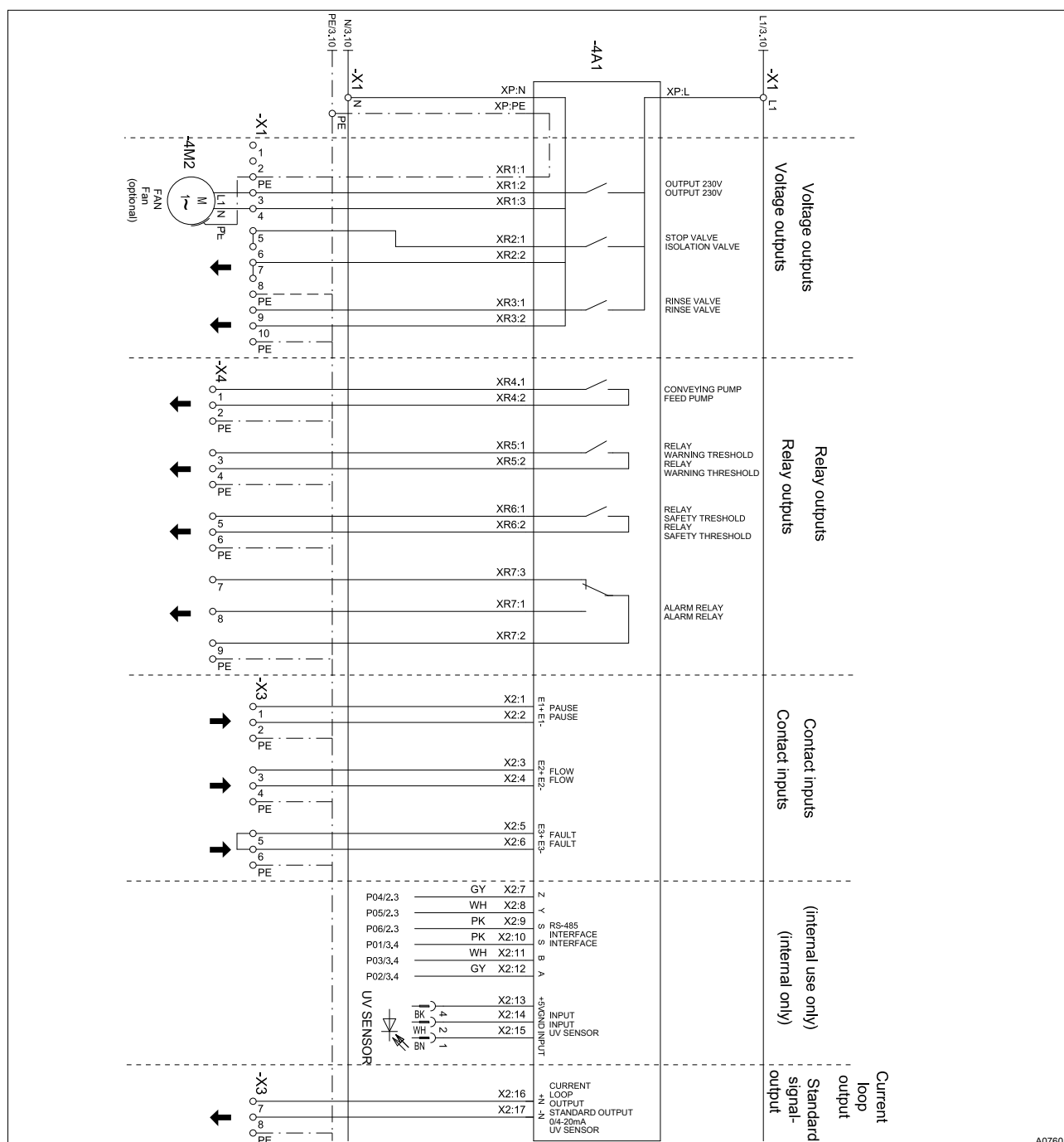
Fig. 57: Terminal Wiring Diagram
