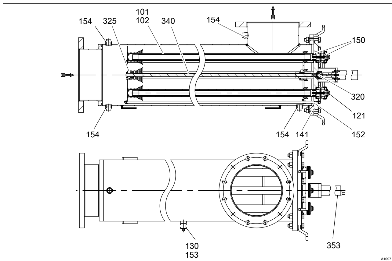
Fig. 55: Spare parts drawing Dulcodes R
