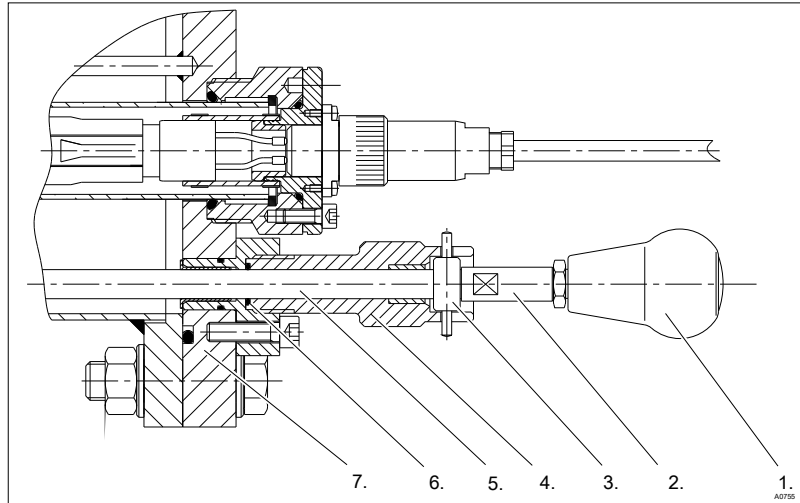
Fig. 32: Components of the manual wiper on the chamber cover
