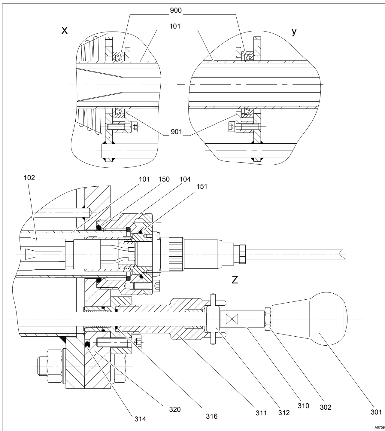
Fig. 54: Details X / Y and cross-section through the lamp connection and manual wiper, spare parts list, see Chapter 10.2 'Spare parts list for UV-systems with manual wiper' on page 77
