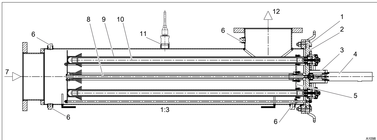
Fig. 29: Construction of the radiation chamber for the example of the Dulcodes 4x300 R with automatic wiper
