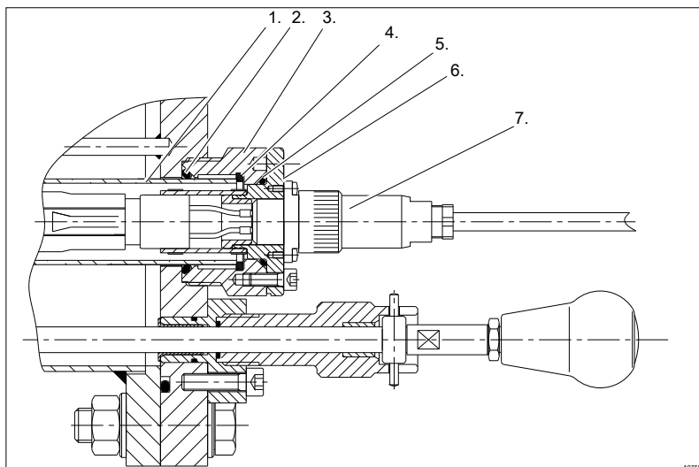
Fig. 34: Cross-section of the lamp connection
