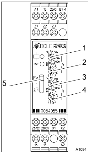
Fig. 31: Pacing relay MK7854N
