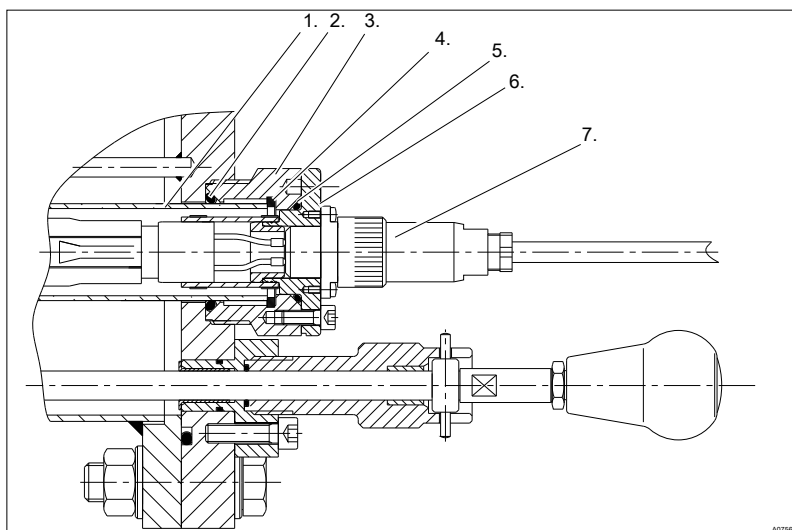
Fig. 38: Cross-section of the lamp connection
