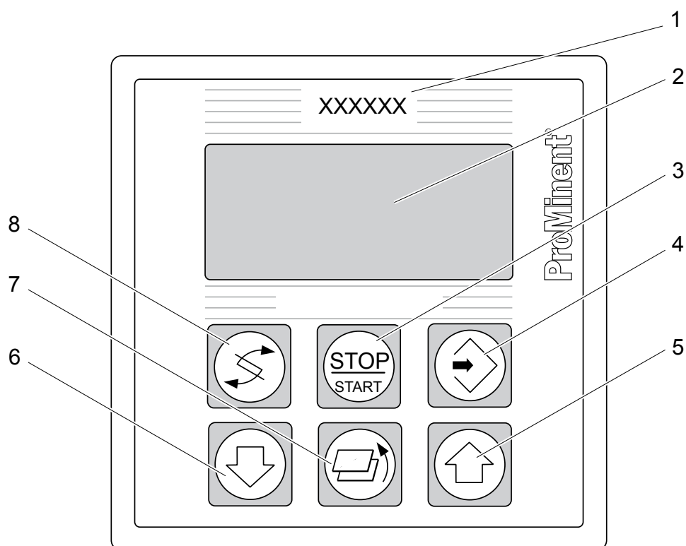
Fig. 2: Display and operating unit
