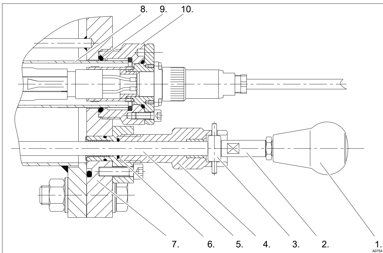
Fig. 30: Components of the manual wiper on the chamber cover and parts of the UV lamp
