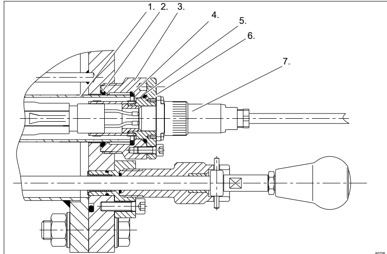
Fig. 33: Cross-section of the lamp connection
