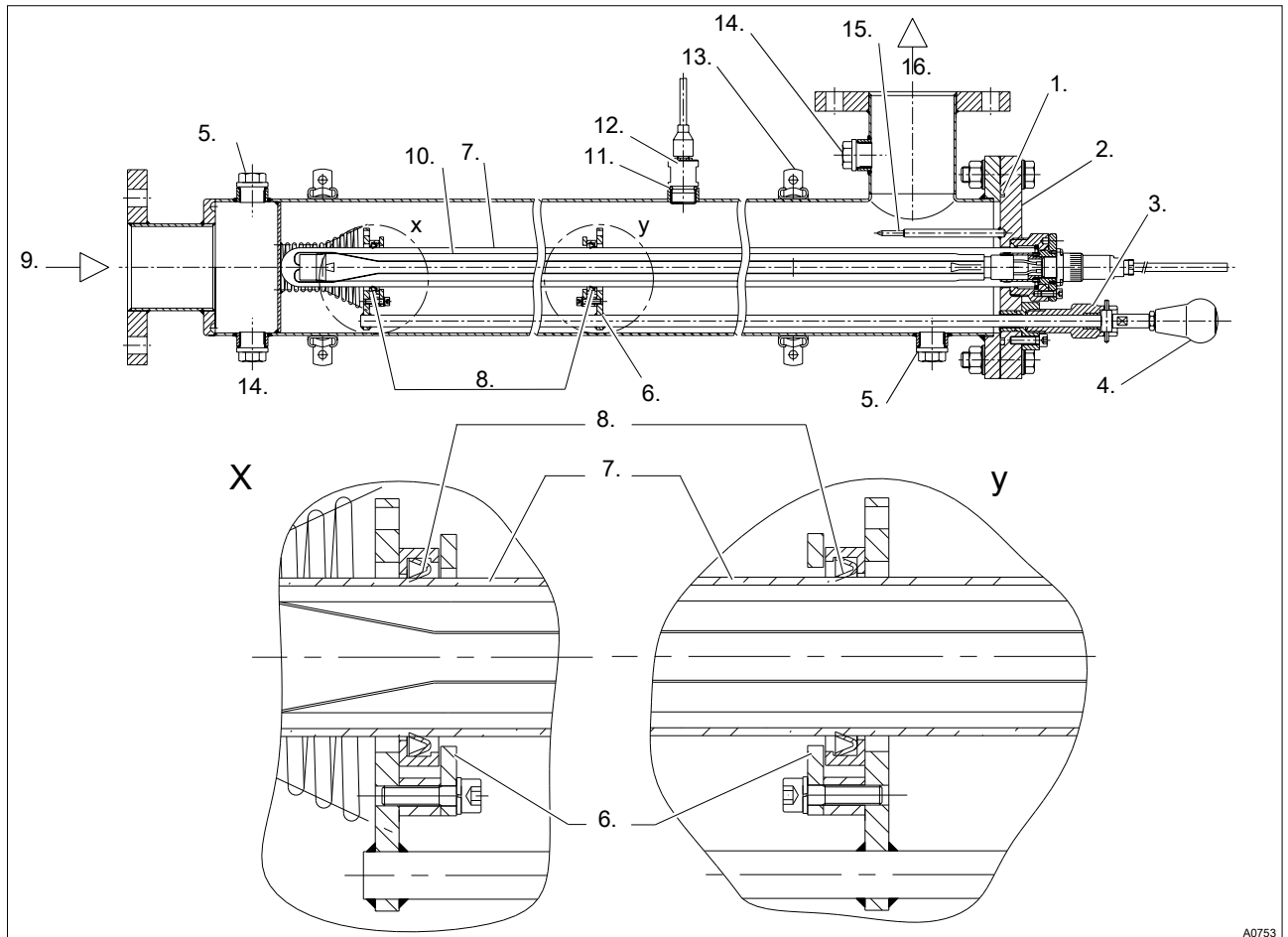
Fig. 28: Construction of the radiation chamber with detail X and Y for the example of a Dulcodes 1x300 R with manual wiper
