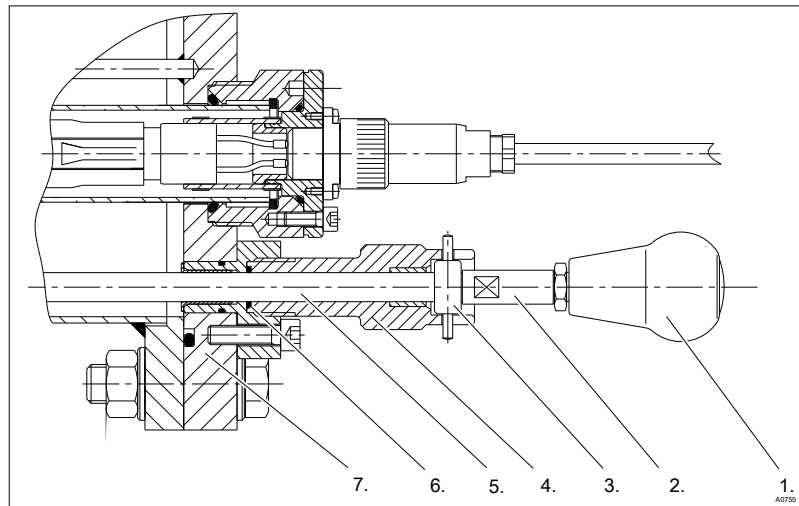
Fig. 35: Components of the manual wiper on the chamber cover
