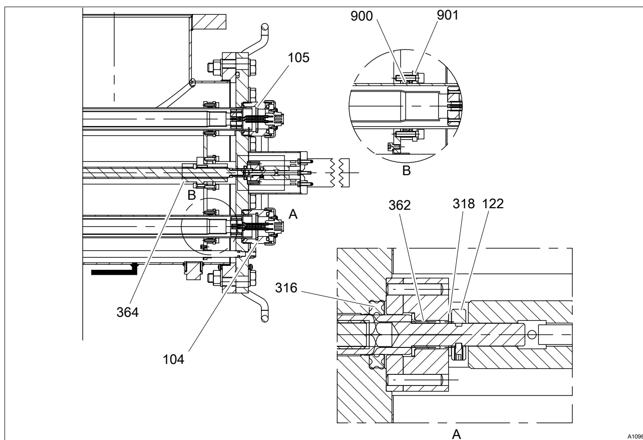
Fig. 56: Details A / B and section through the lamp connection and automatic wiper
