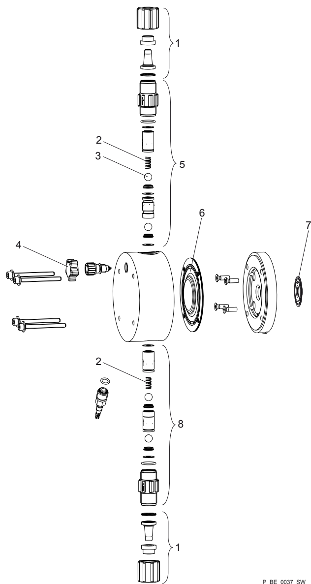
Fig. 6: Beta® 0232 NP liquid end with and without bleed valve
