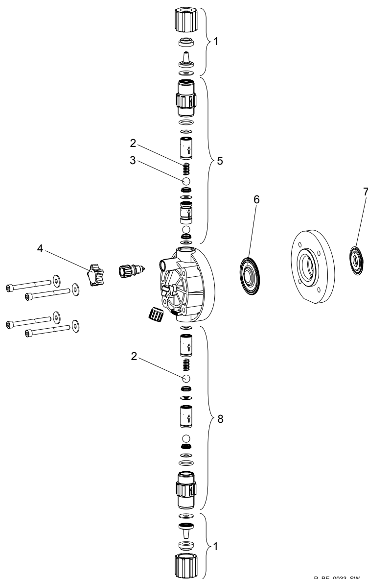
Fig. 8: Beta® 0708 (1008) - 0220 (0420) PV liquid end with bleed valve
