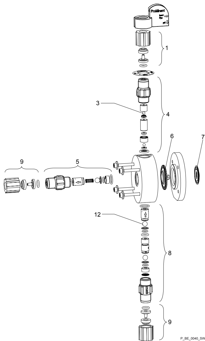
Fig. 18: Beta® 0708 (1008) - 0220 (0420) PP / NP SEK liquid end, self-bleeding
