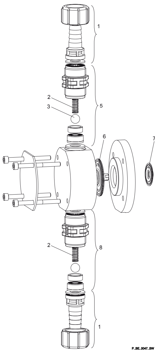
Fig. 10: Beta® 1604 - 0220 (0420) PV HV liquid end, for highly viscous feed chemicals
