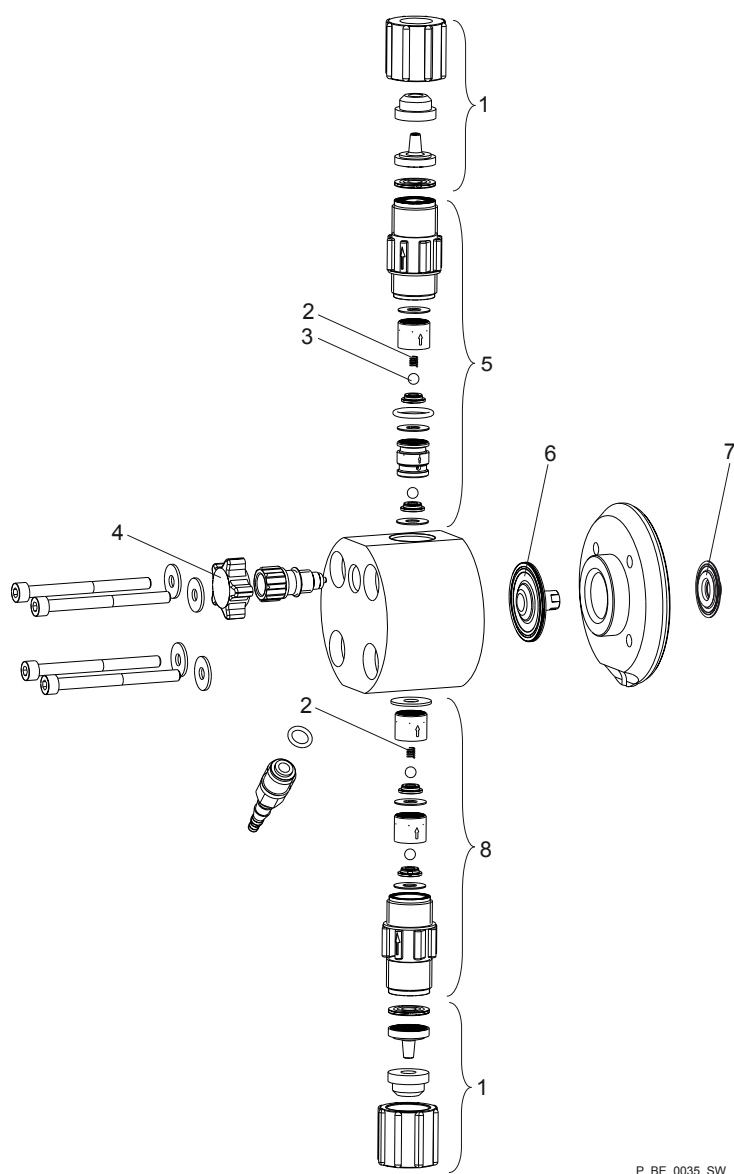
Fig. 4: Beta® 1000 - 1604 NP liquid end with and without bleed valve
