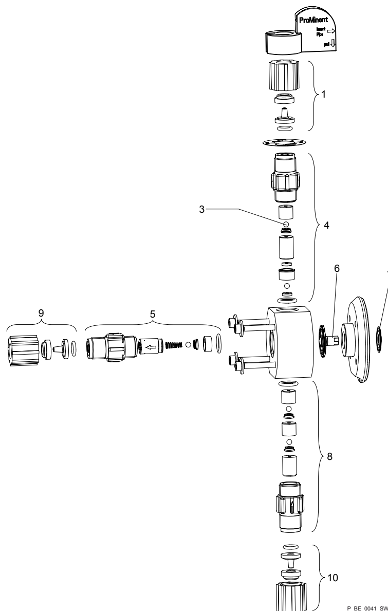
Fig. 17: Beta® 1601 - 1604 PP SEK and 1601 - 1604 NP SEK liquid end, self-bleeding
