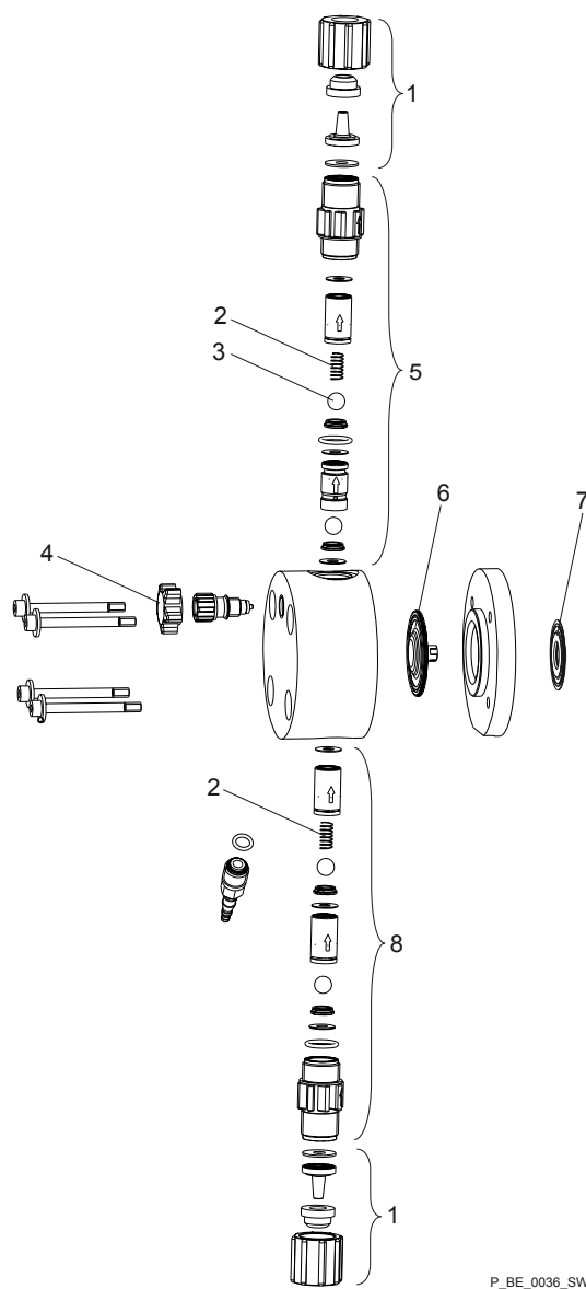
Fig. 5: Beta® 0708 (1008) - 0220 (0420) NP liquid end with and without bleed valve
