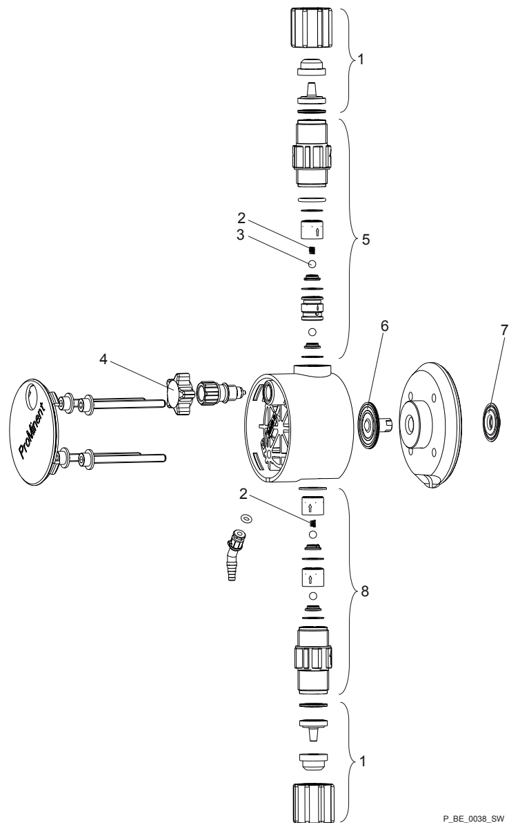
Fig. 1: Beta® 1000 - 1604 PP liquid end with bleed valve
