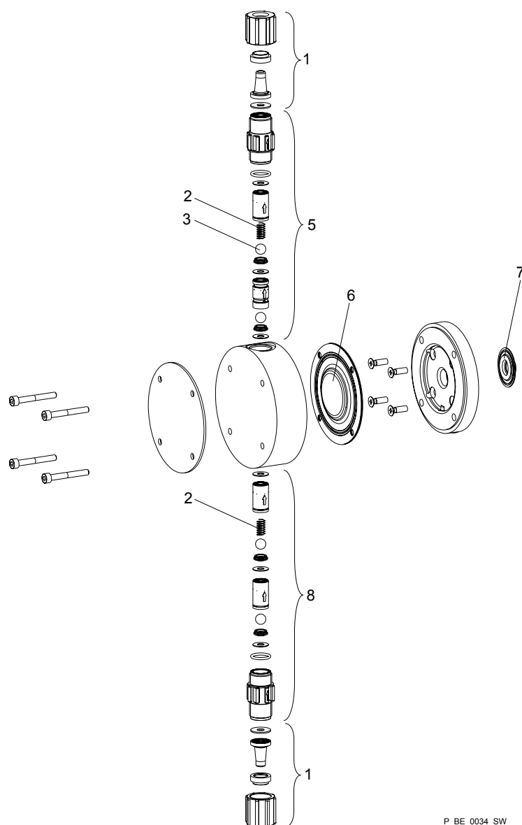
Fig. 3: Beta® 0232 PP liquid end without bleed valve
