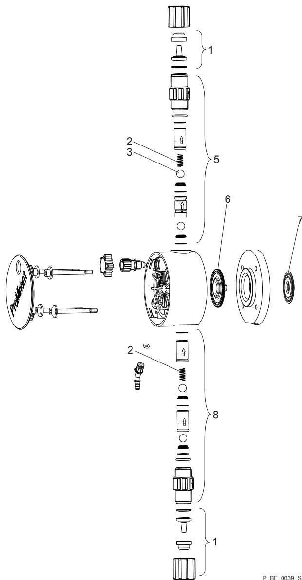
Fig. 2: Beta® 0708 (1008) - 0220 (0420) PP liquid end with bleed
