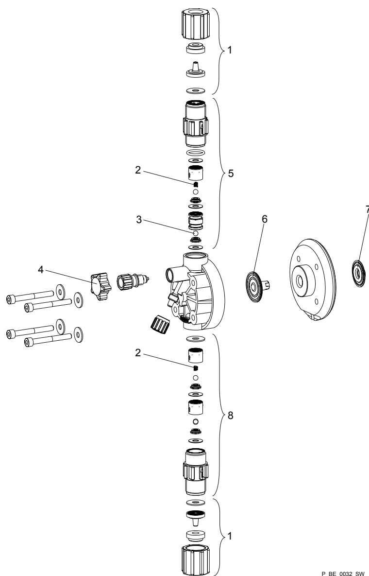
Fig. 7: Beta® 1000 - 1604 PV liquid end with bleed valve
