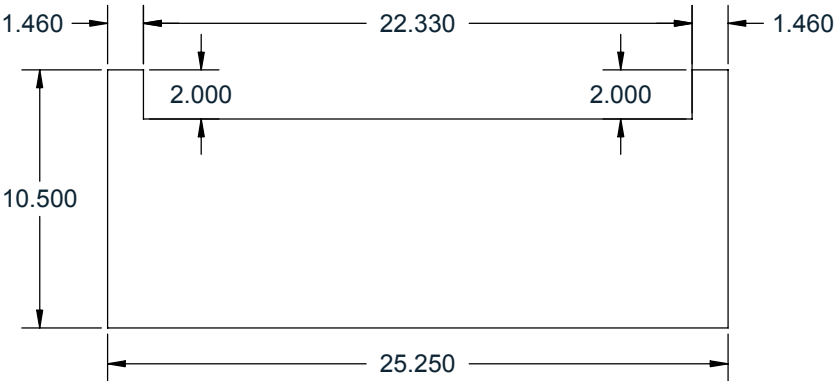
SUPPORT PANEL DETAIL
