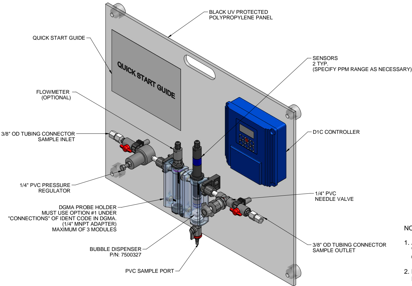
ISOMETRIC VIEW
