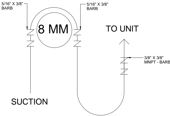
PUMP LAYOUT
