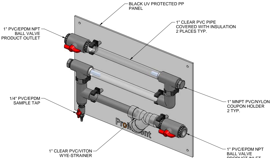
ISOMETRIC VIEW
