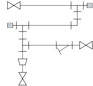
PIPING SCHEMATIC
