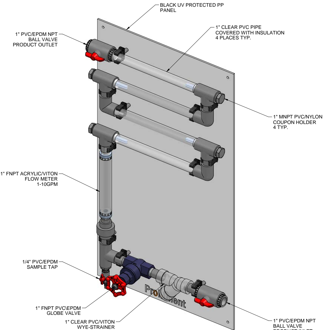
ISOMETRIC VIEW
