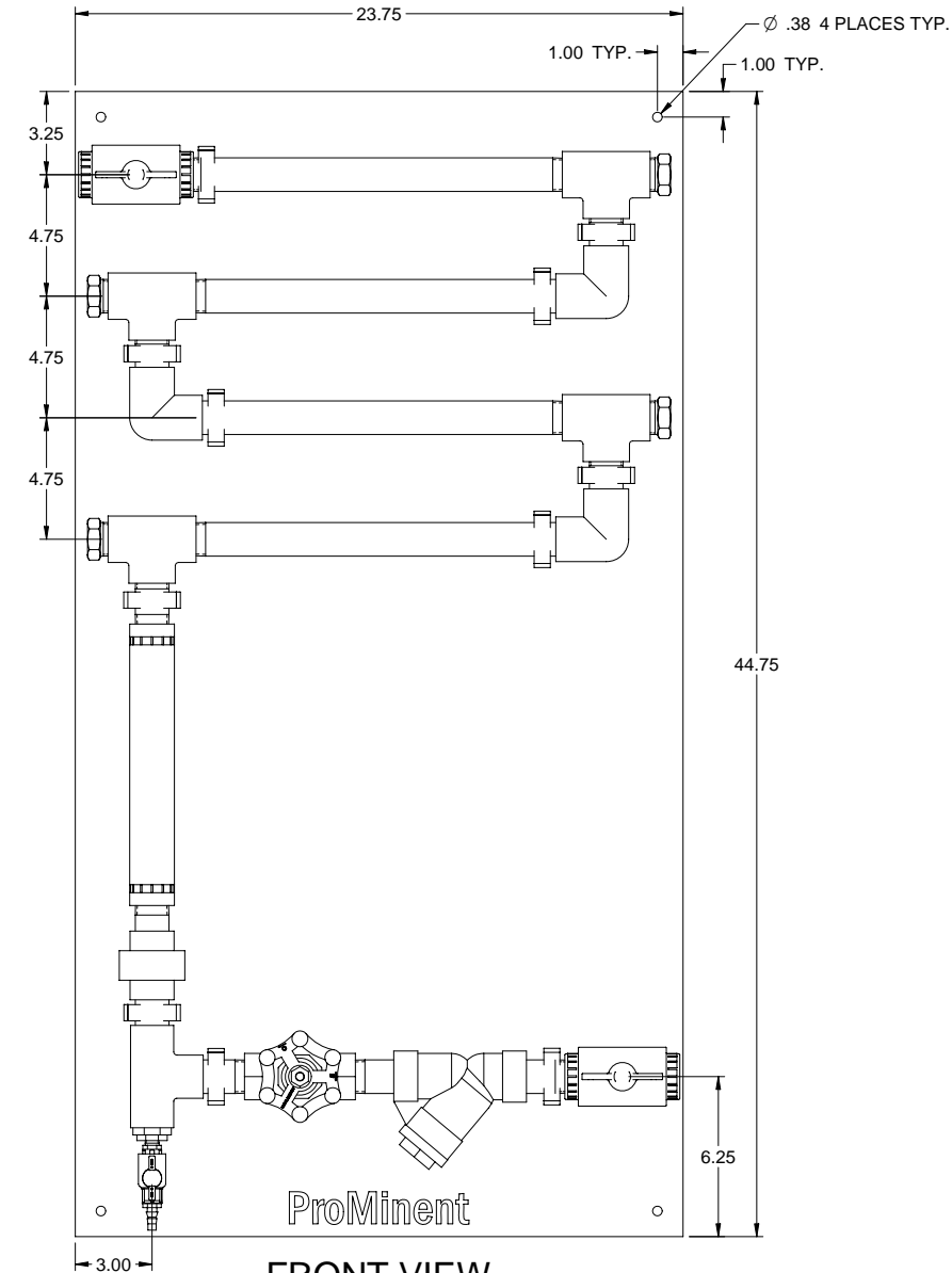
FRONT VIEW
