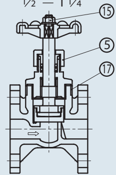
FLANGED 1/2" — 1 1/4"
