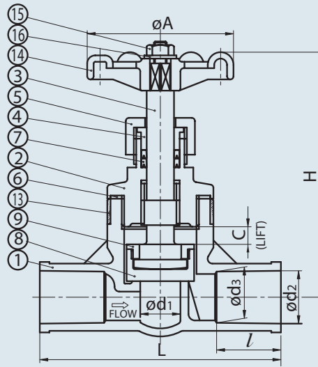
SOCKET END 1/2" — 1 1/4"
