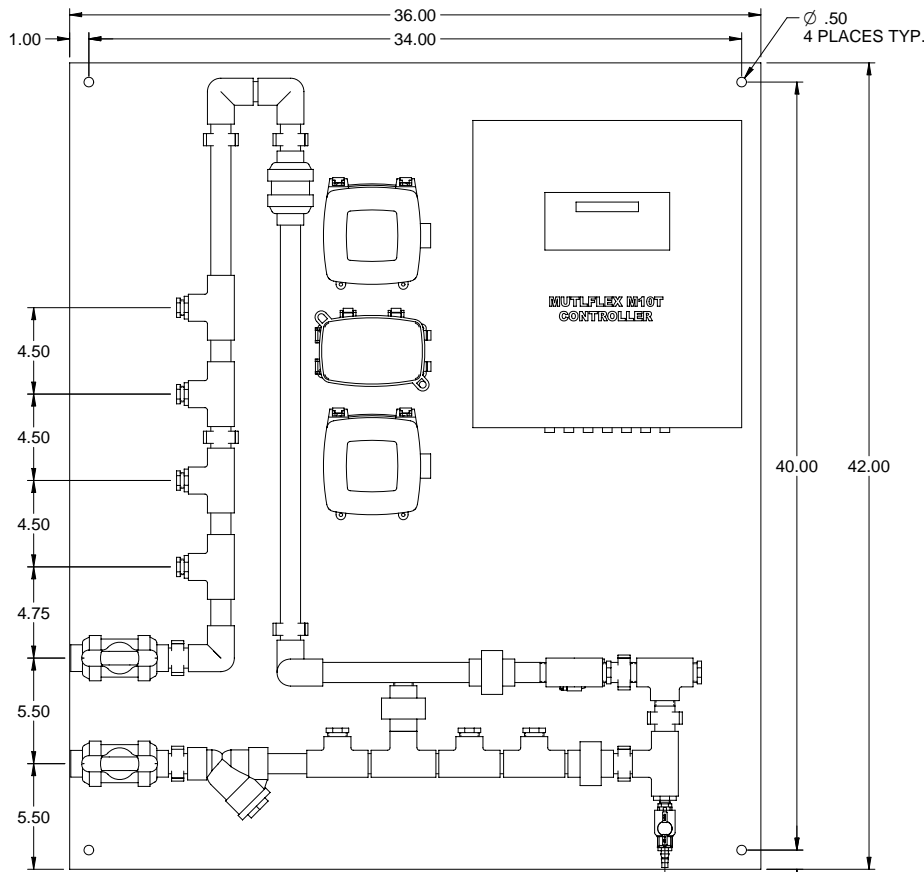
FRONT VIEW
