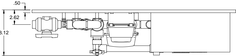
PLAN VIEW
