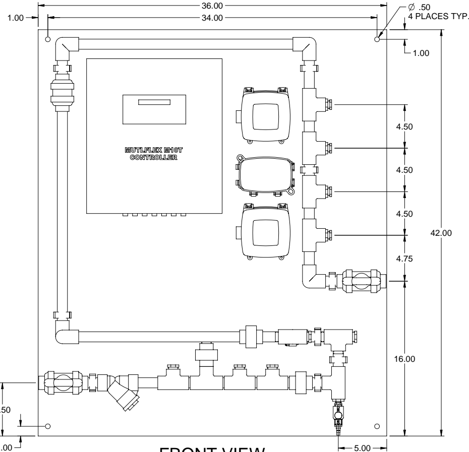
FRONT VIEW
