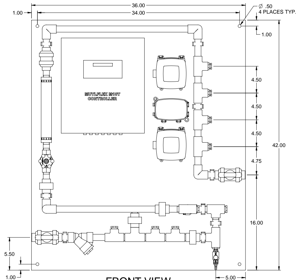
FRONT VIEW
