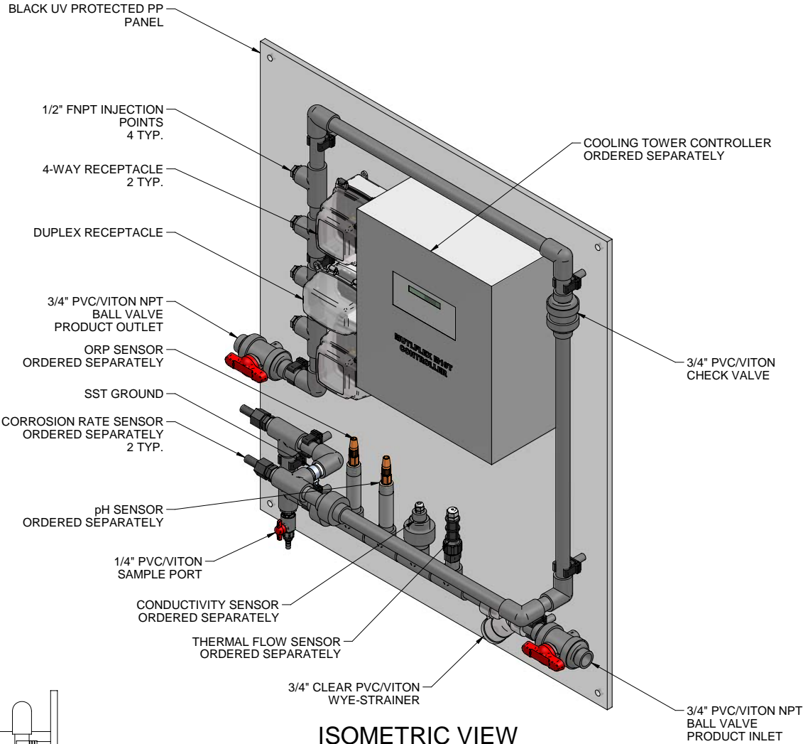
ISOMETRIC VIEW SHOWN WITH SENSORS MOUNTED
