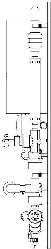
SIDE VIEW
