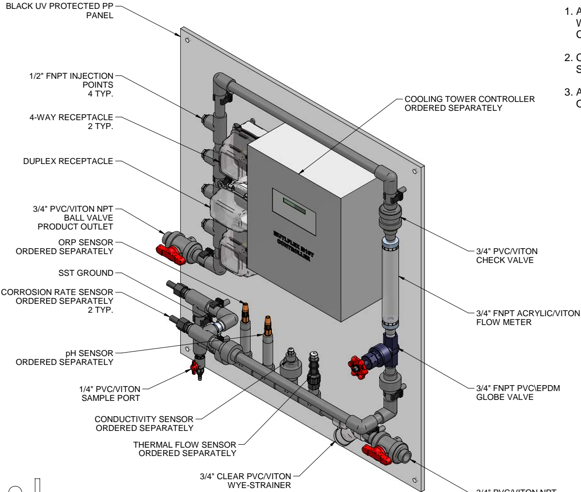
ISOMETRIC VIEW SHOWN WITH SENSORS MOUNTED
