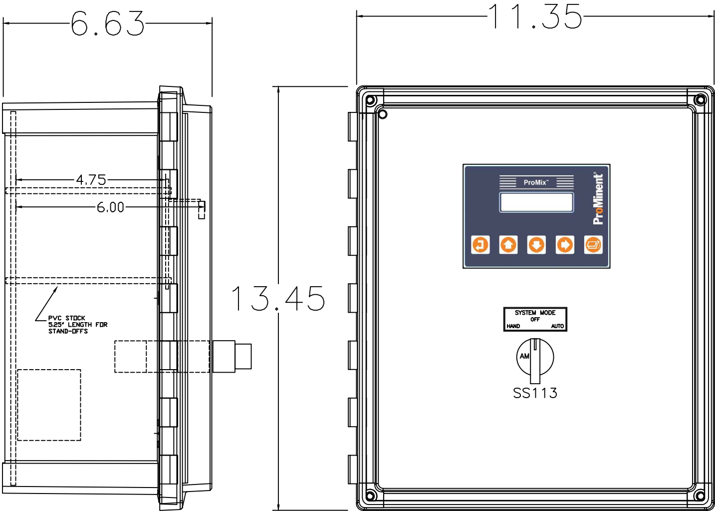
FIBOX 12106 POLYCARBONATE ENCLOSURE
