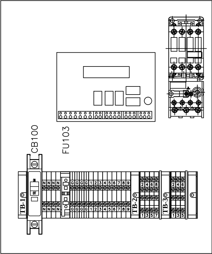
FIBOX 12X10 SUB PANEL
