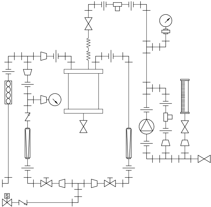
PIPING SCHEMATIC
