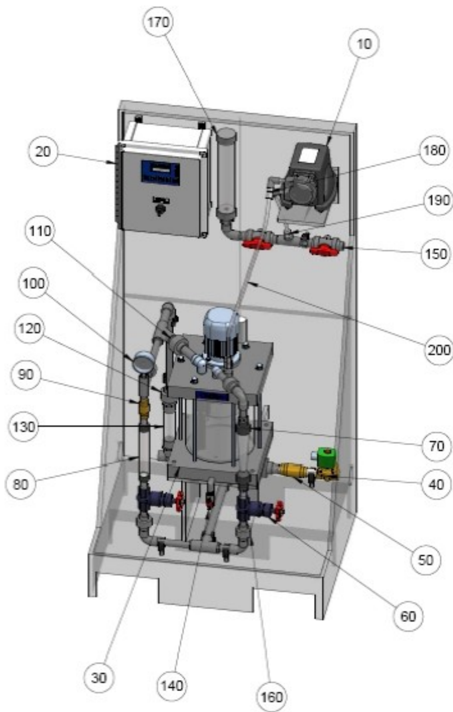
PROMIX S CONTROL A
