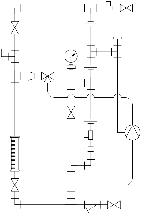
PIPING SCHEMATIC
