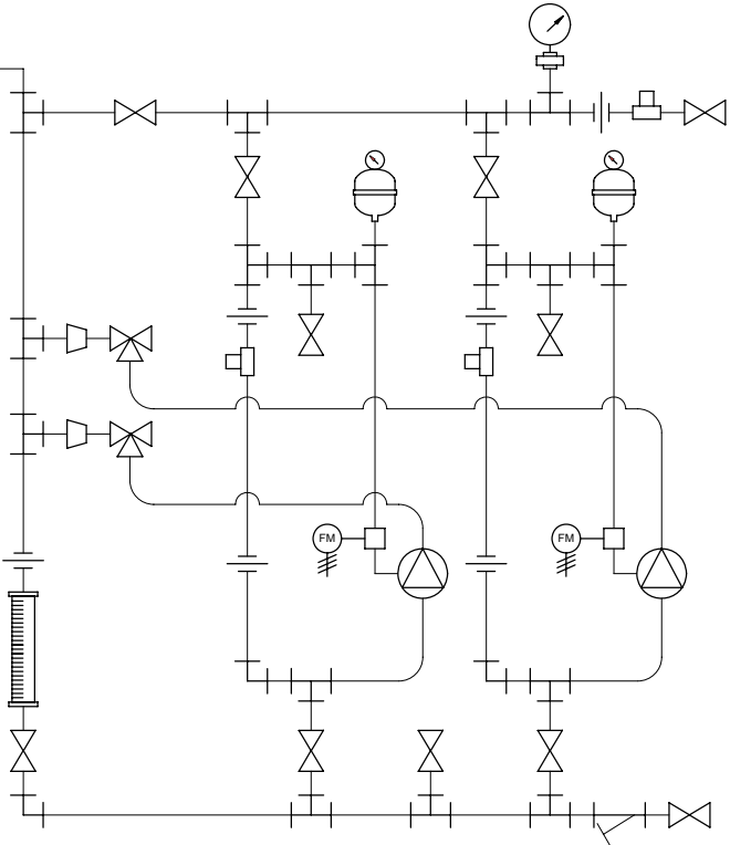
PIPING SCHEMATIC
