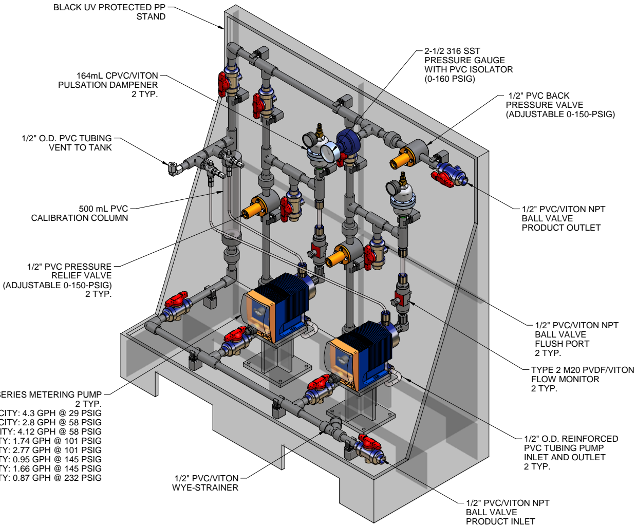
ISOMETRIC VIEW
