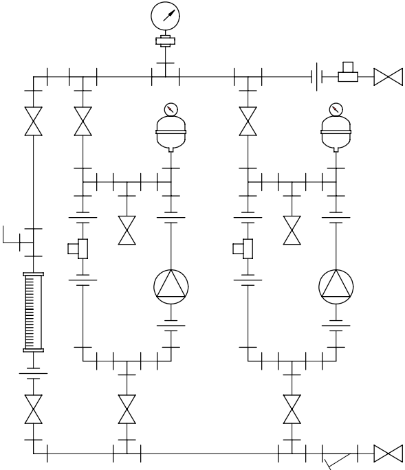
PIPING SCHEMATIC
