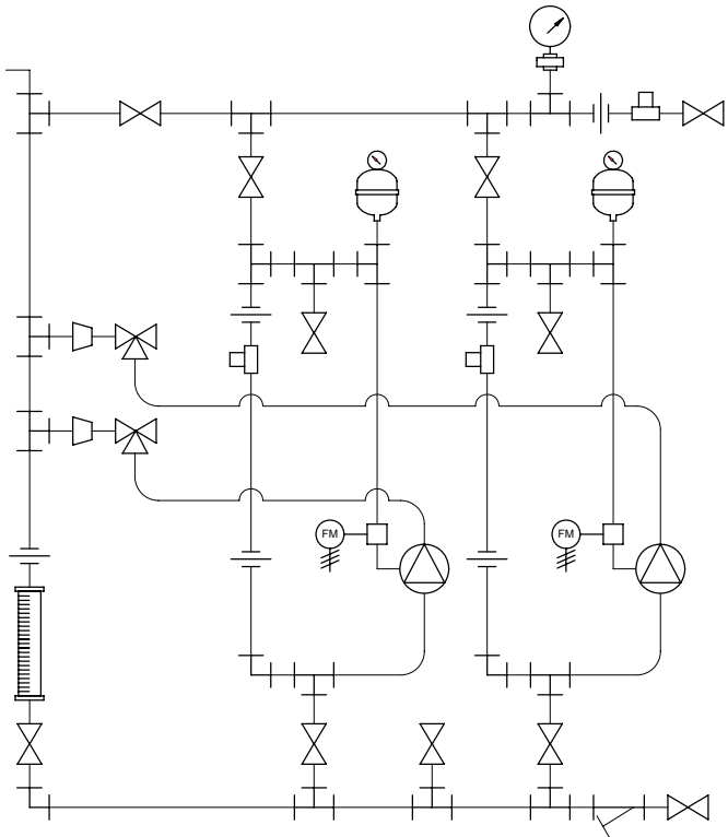
PIPING SCHEMATIC
