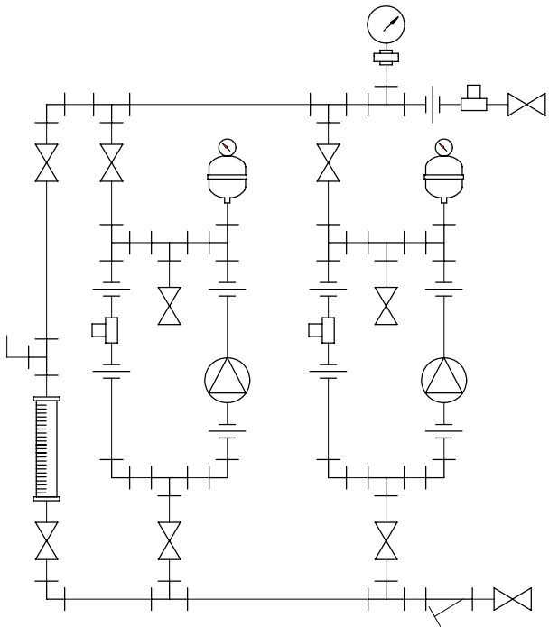
PIPING SCHEMATIC
