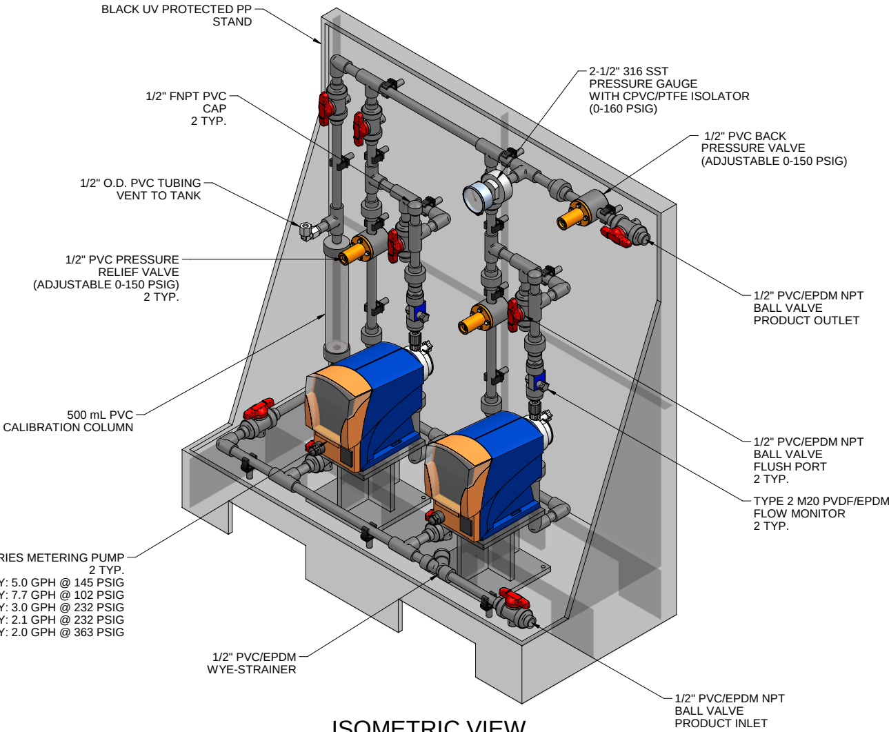
ISOMETRIC VIEW
