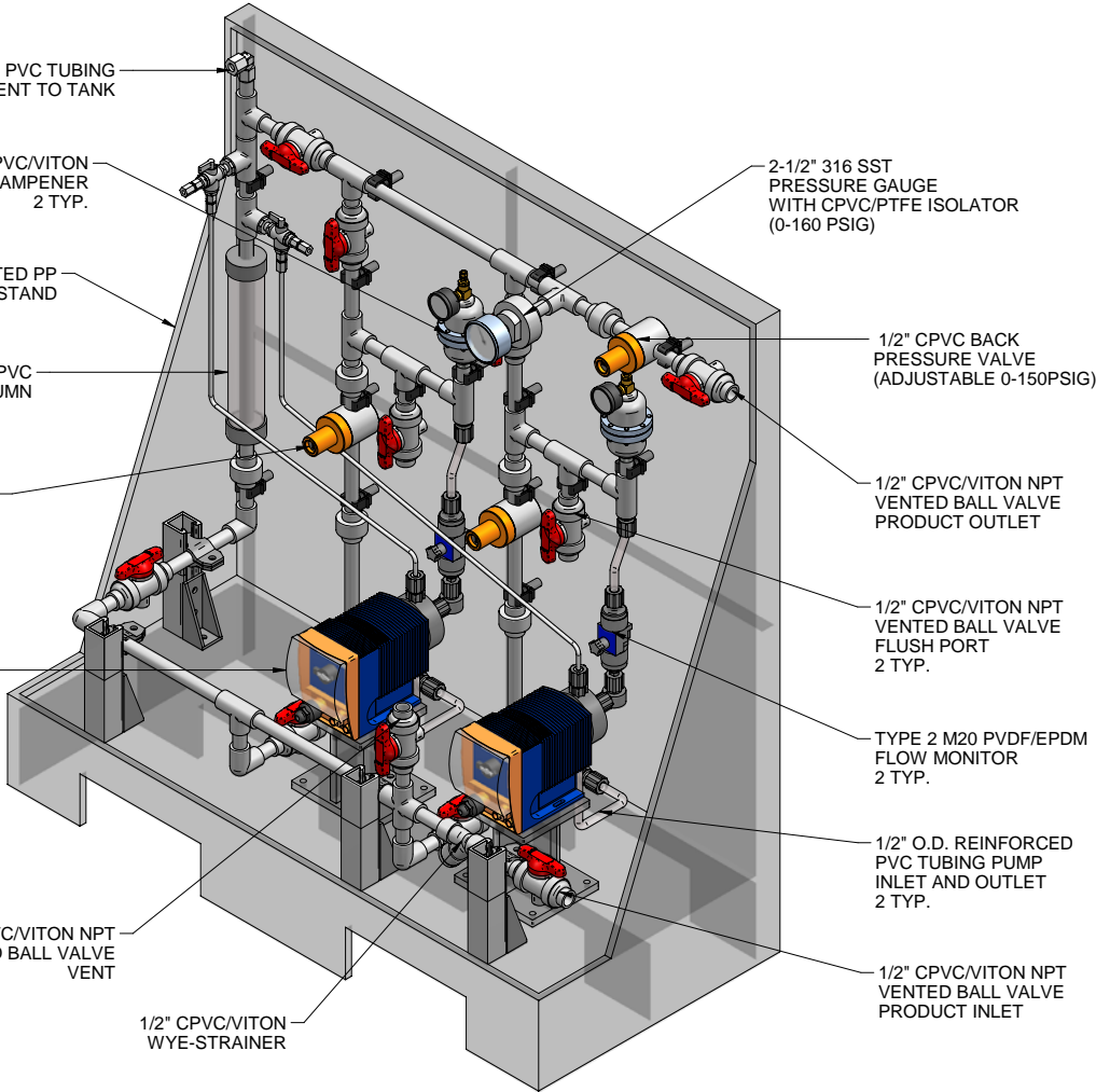
ISOMETRIC VIEW
