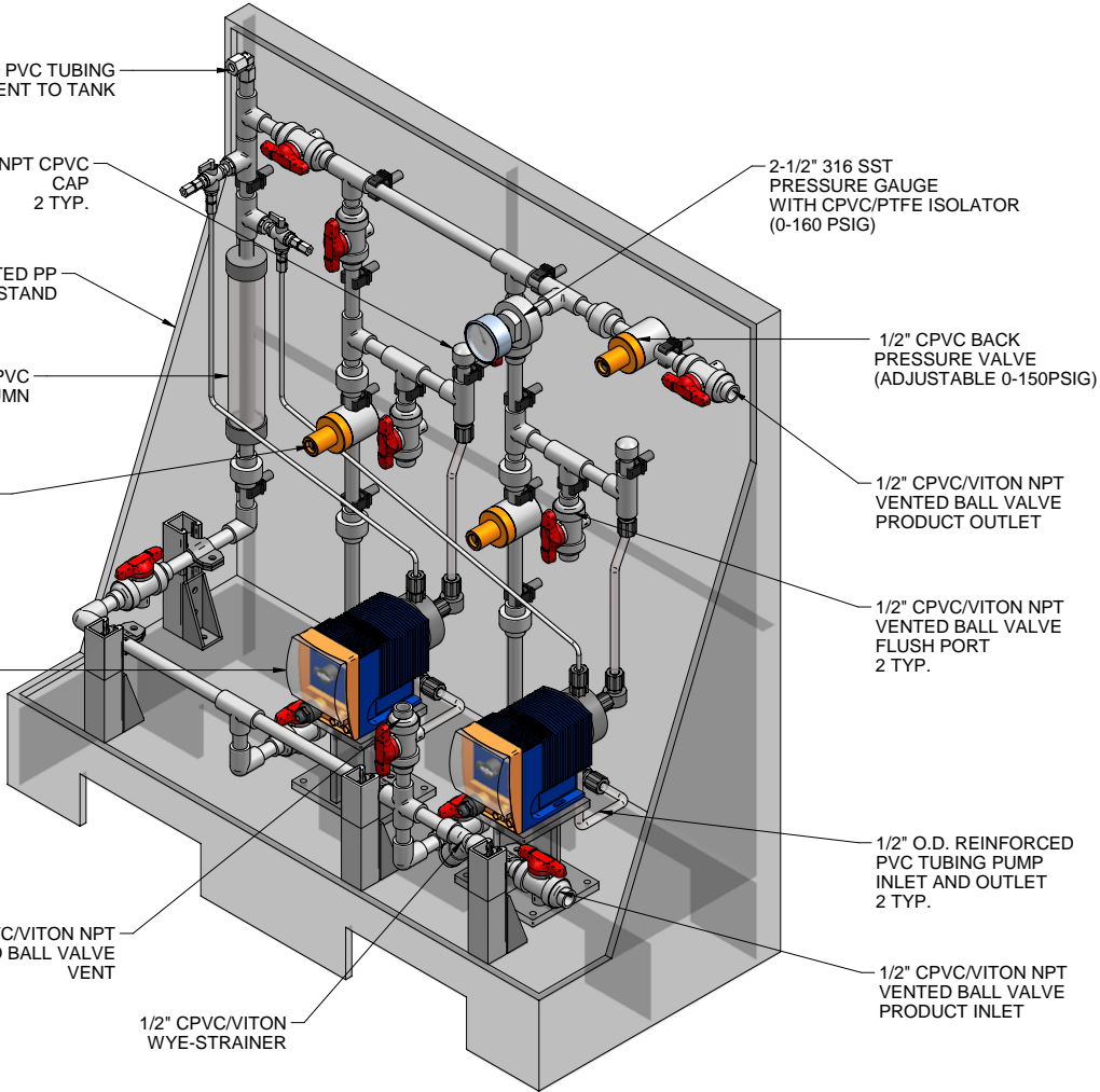
ISOMETRIC VIEW
