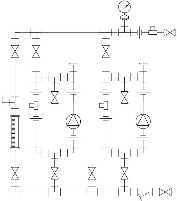
PIPING SCHEMATIC
