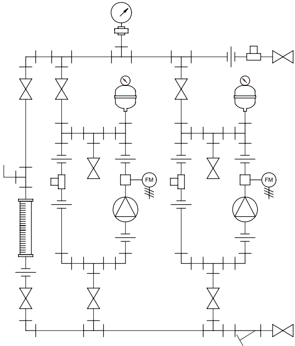
PIPING SCHEMATIC
