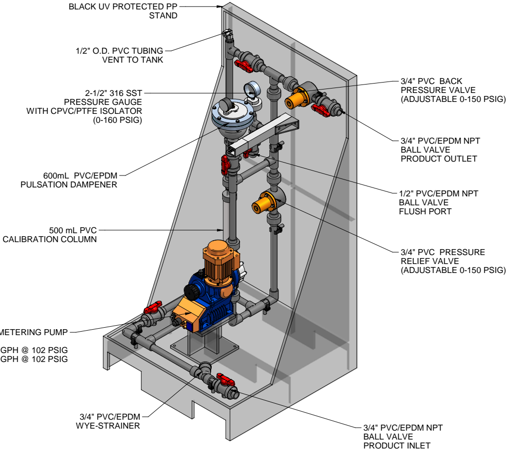
ISOMETRIC VIEW
