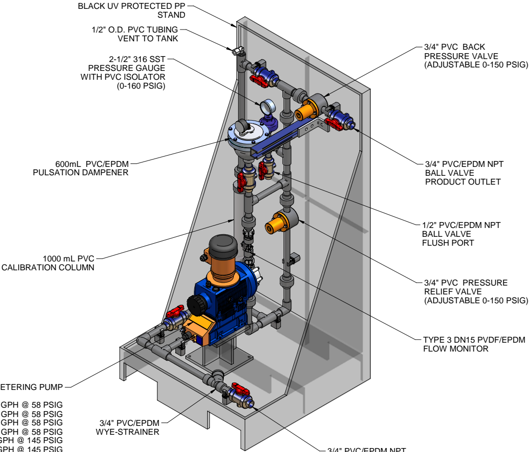
ISOMETRIC VIEW
