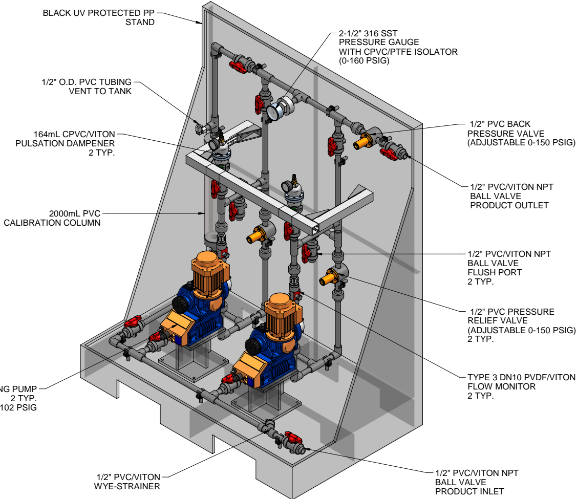
ISOMETRIC VIEW
