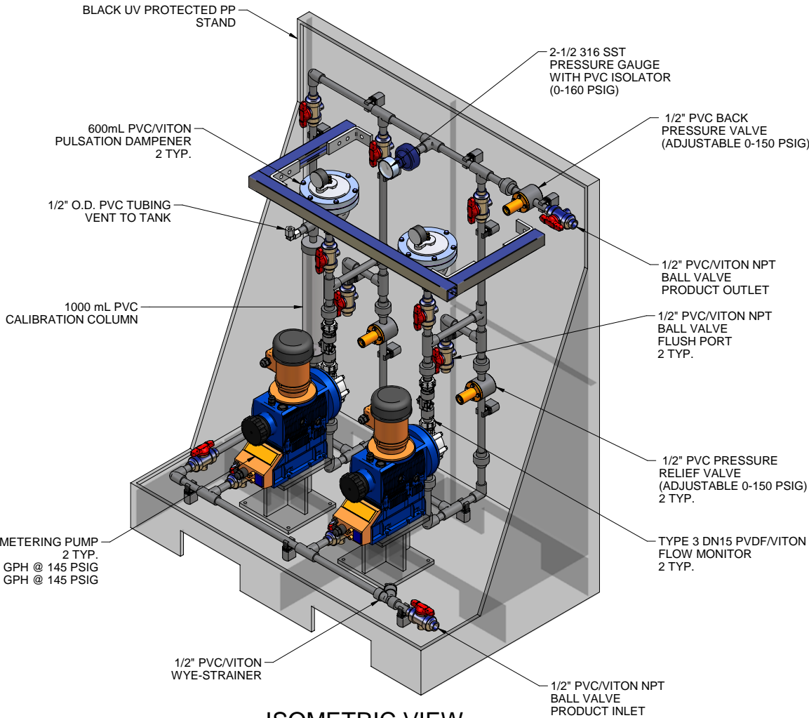
ISOMETRIC VIEW
