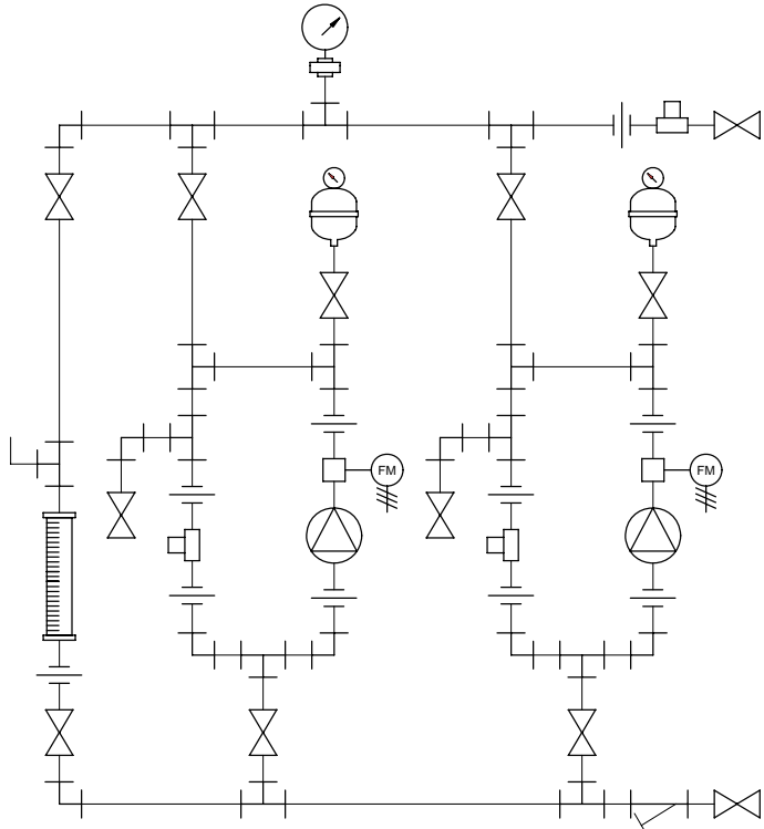
PIPING SCHEMATIC
