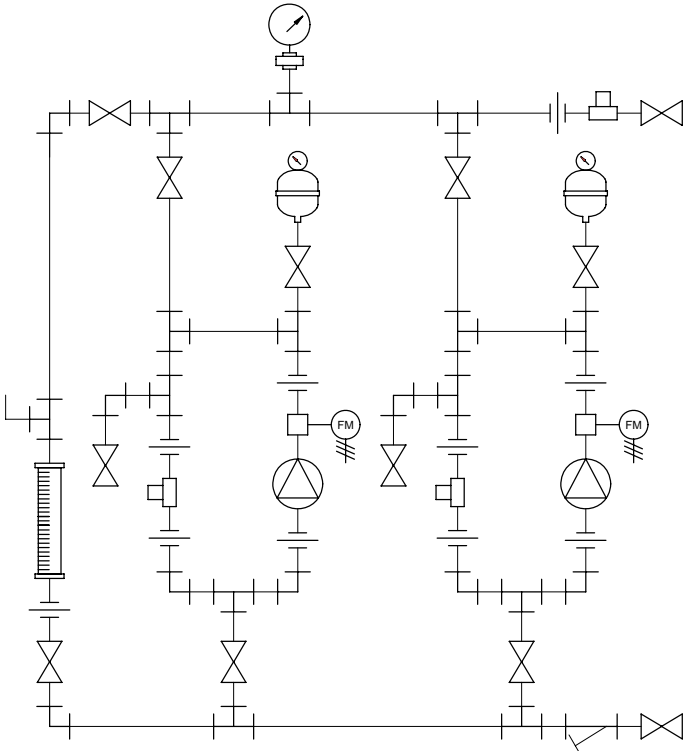
PIPING SCHEMATIC
