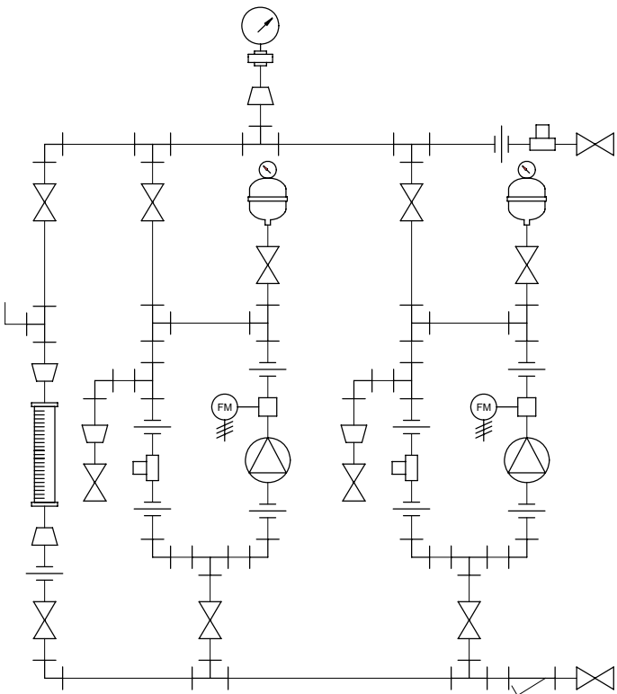
PIPING SCHEMATIC
