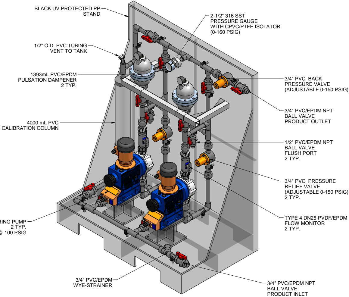
ISOMETRIC VIEW
