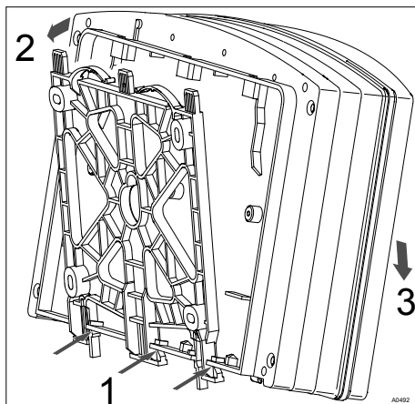
Fig. 11: Fitting the wall bracket
