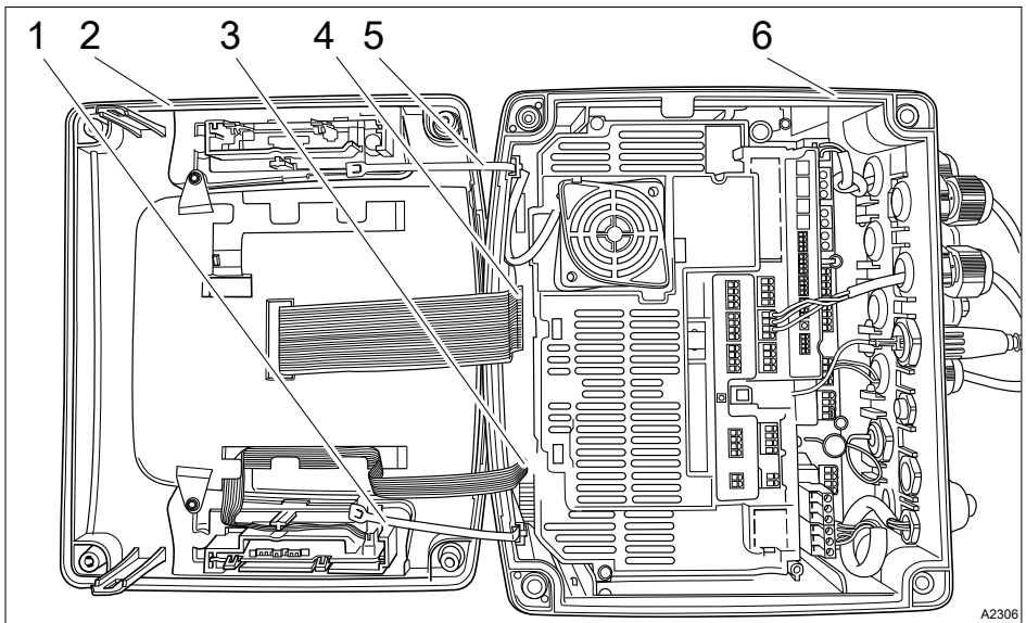
Fig. 112: Replacement of spare parts units
