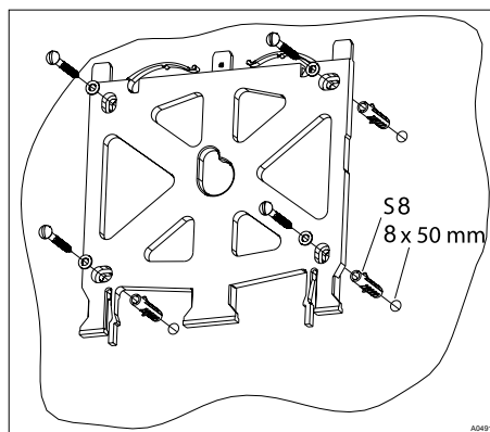
Fig. 10: Fitting the wall bracket
