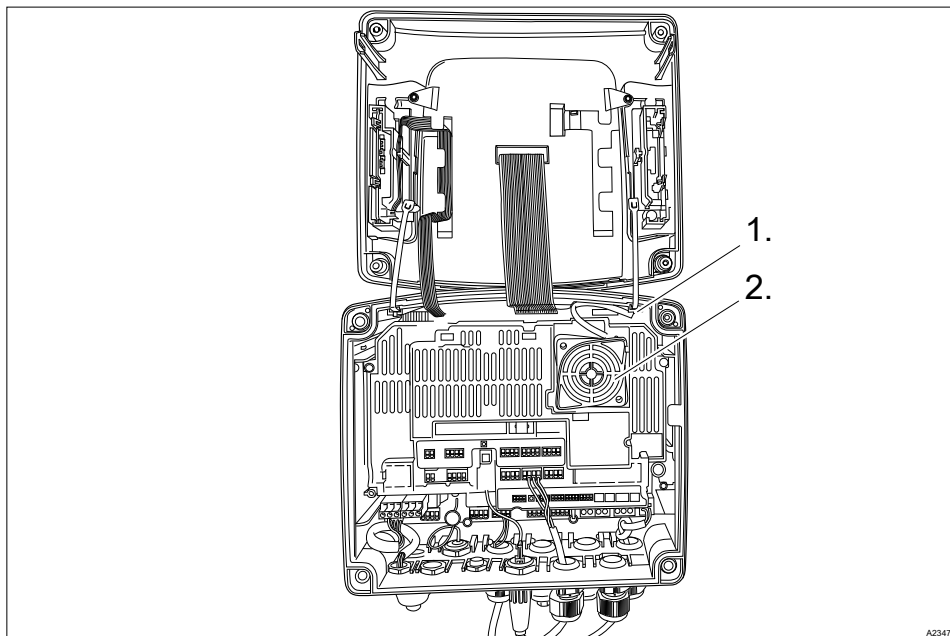
Fig. 113: Replacing a fan, part no. 733328
