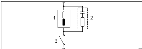
Fig. 26: RC protective circuit for the relay contacts
