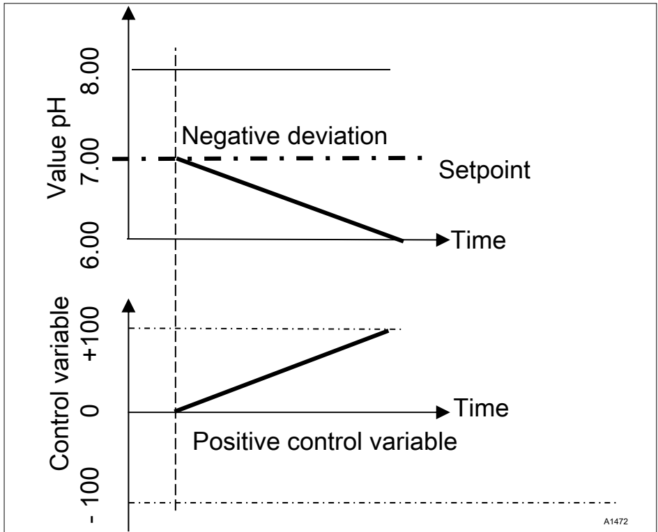
Fig. 73: Control type PID monodirectional, pH-increasing direction
