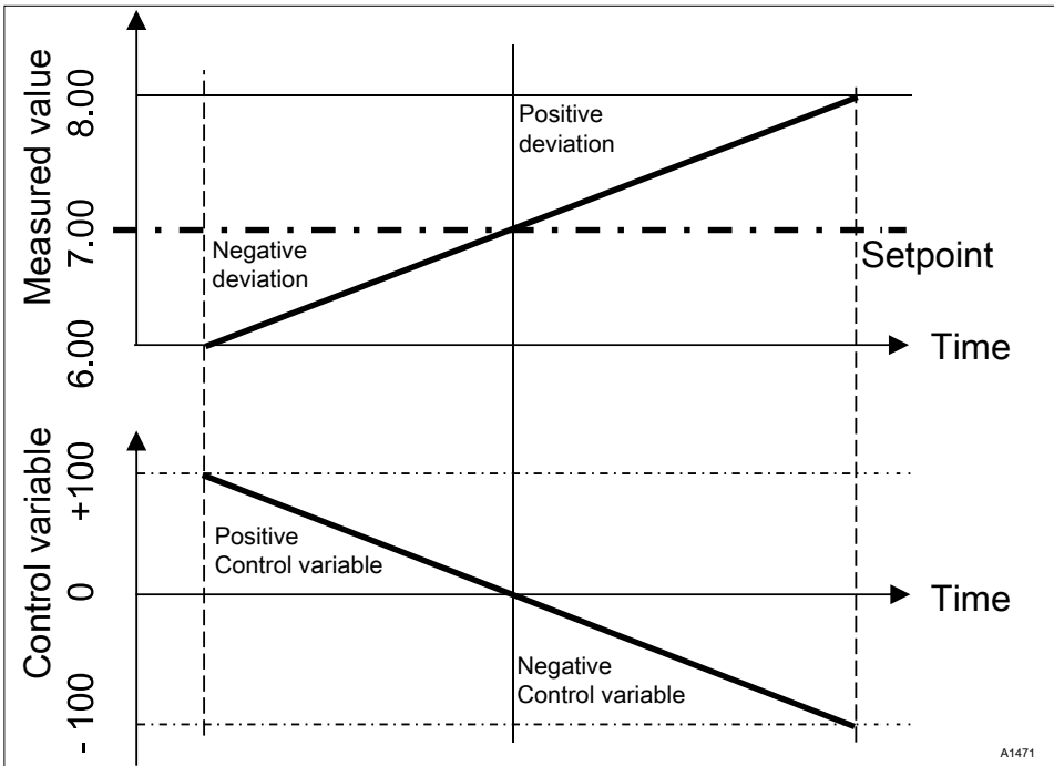
Fig. 70: Control type PID bidirectional. Control characteristic without dead zone
