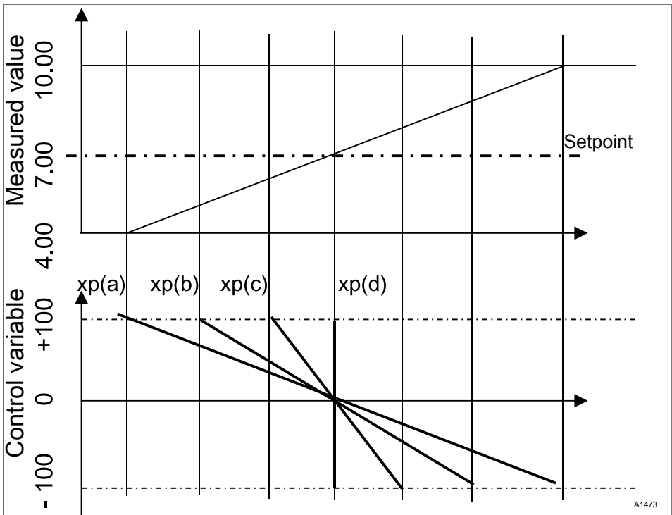
Fig. 74: The smaller the xp value, the more "forcefully" the control reacts.
