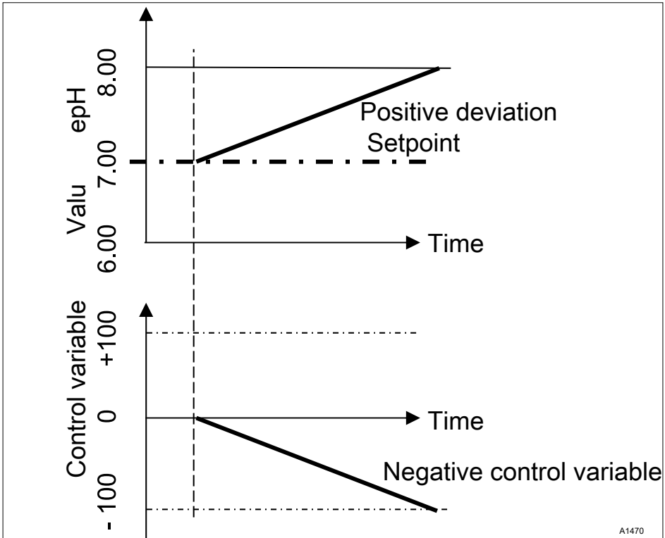
Fig. 72: Control type PID monodirectional, pH-lowering direction
