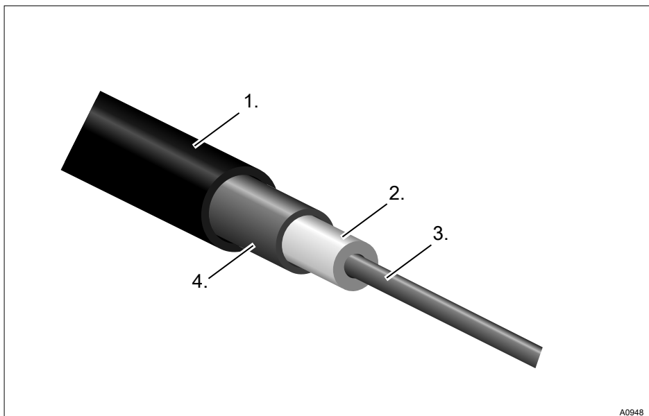
Fig. 27: Coaxial cable:
