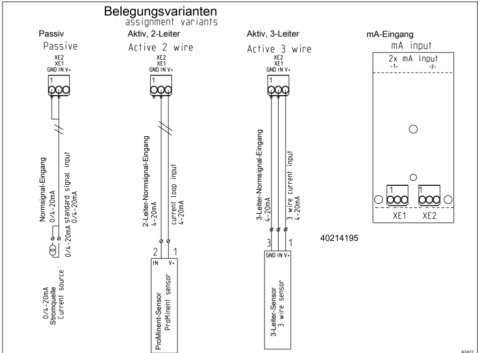
Fig. 24: Module: 2x mA inputs. Part number 734126
