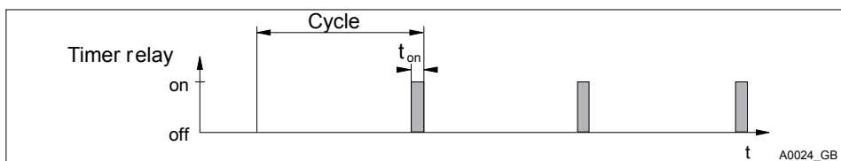
Fig. 90: Timer relay
