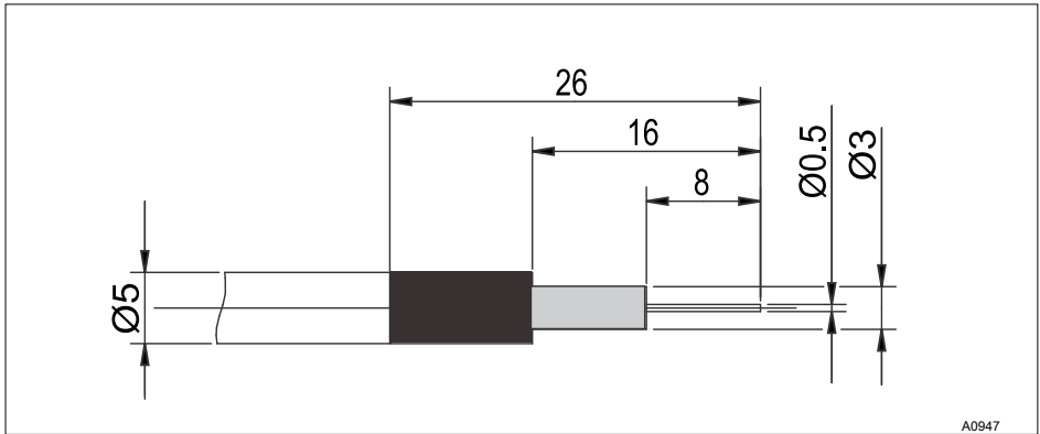
Fig. 28: Coaxial cable assembly
