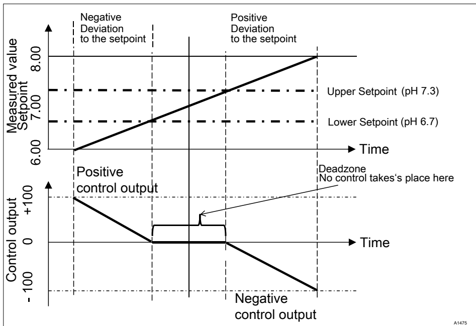
Fig. 71: Control type PID bidirectional, with dead zone
