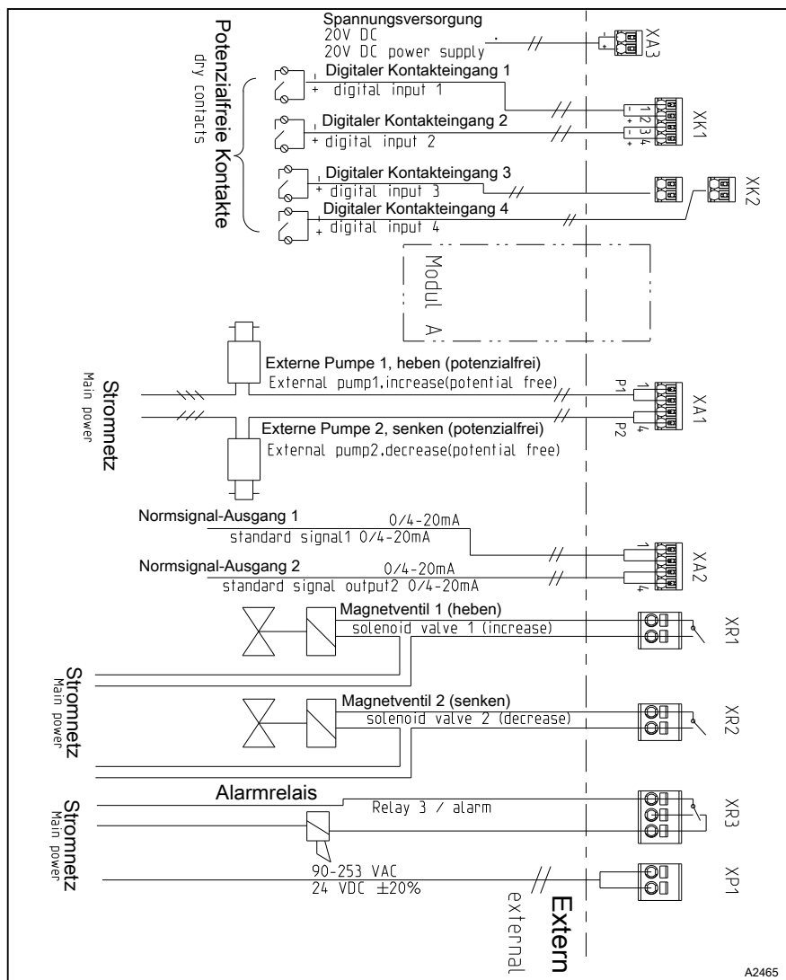
Fig. 16: Terminal diagram with assignment options. Base module channel 1 and 2, there can only be one main measured variable, e.g. chlorine sensor connected to a unit.
