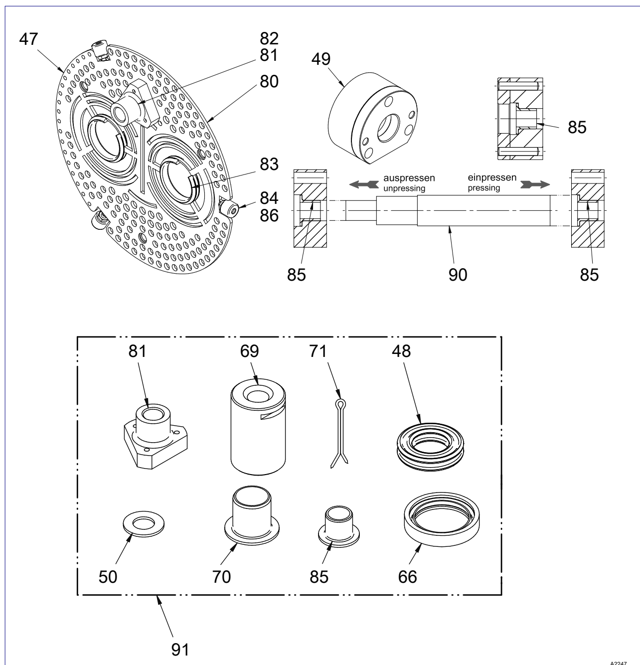
Fig. 63: Spare part diagram, 2 ... 4x350 W, multiple lamp system with wiper
