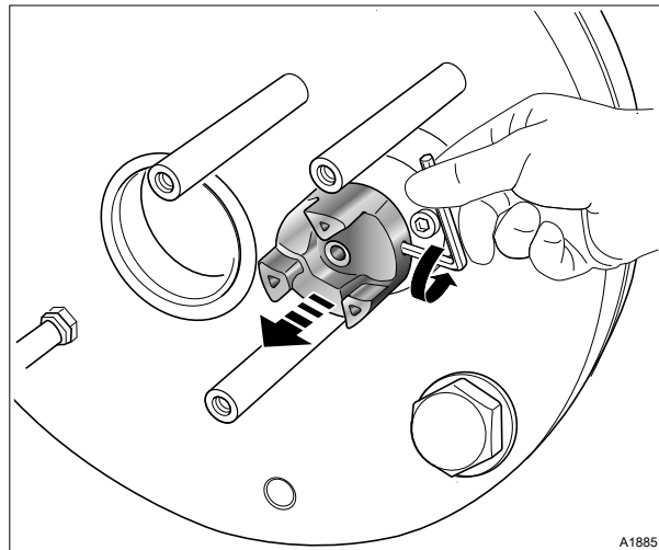
Fig. 16: Coupling / Splint
