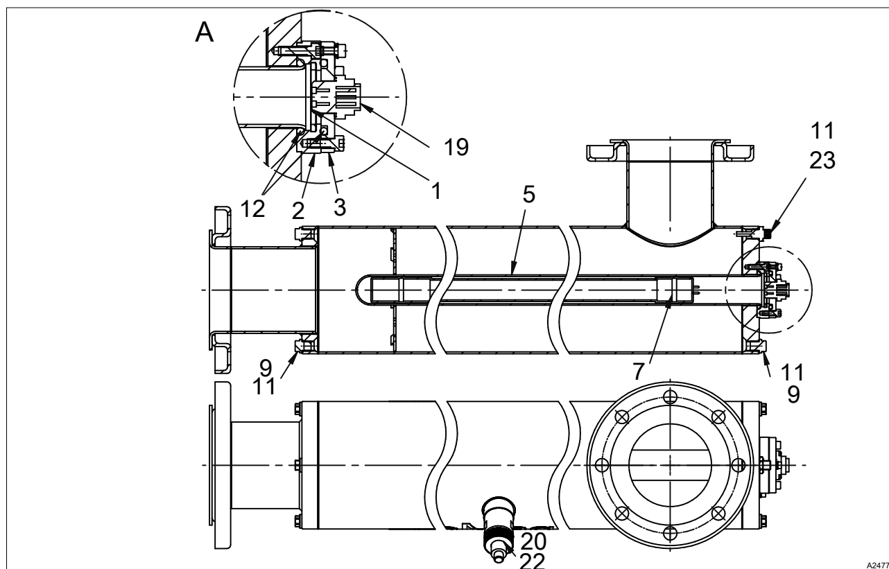
Fig. 51: Spare parts, 350 W, single lamp system without wiper
