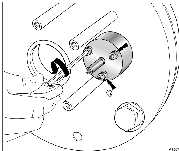
Fig. 18: Bearing cover
