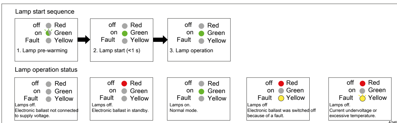
Fig. 4: Operating status and LED displays of lamp operation equipment.
