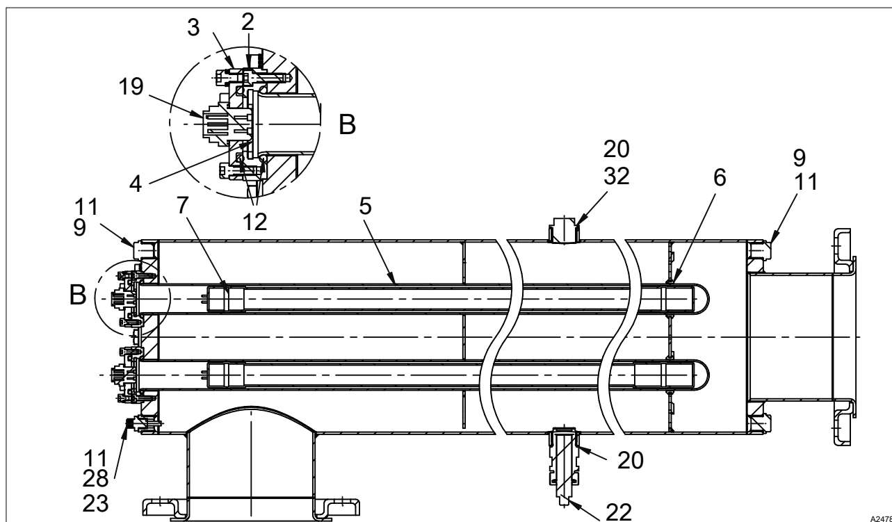
Fig. 52: Spare parts, 2x350 W, UV two lamp system without wiper
