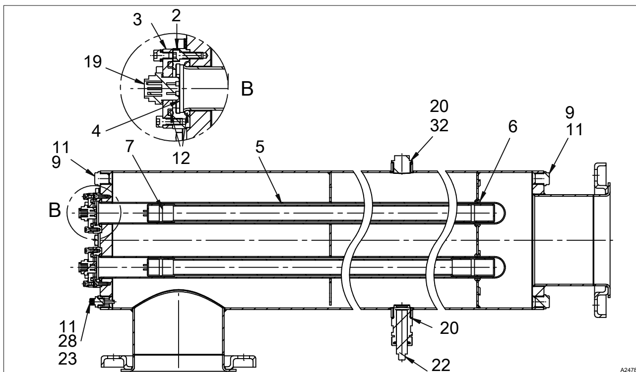
Fig. 55: Spare parts, 4x350 W, UV four lamp system without wiper
