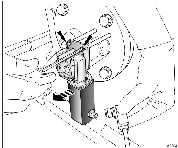
Fig. 11: Flange plate
