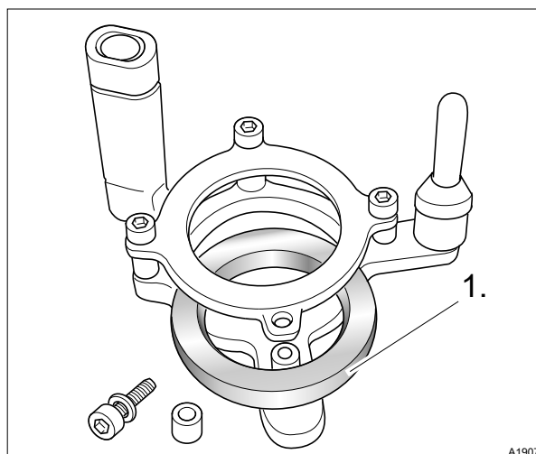
Fig. 38: Wiper element (1)
