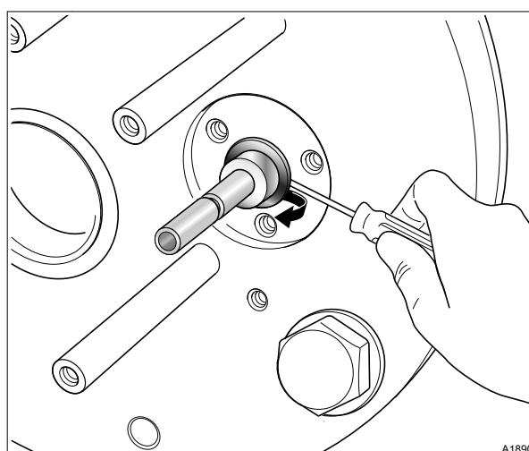
Fig. 20: X-ring
