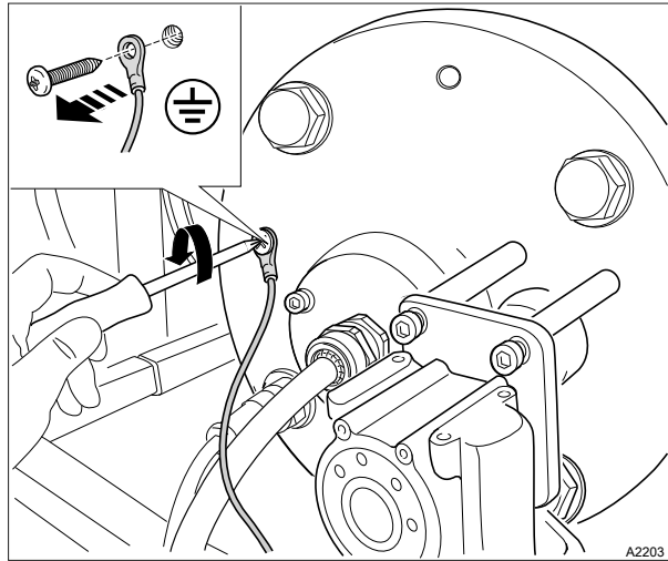
Fig. 10: Earthing cable
