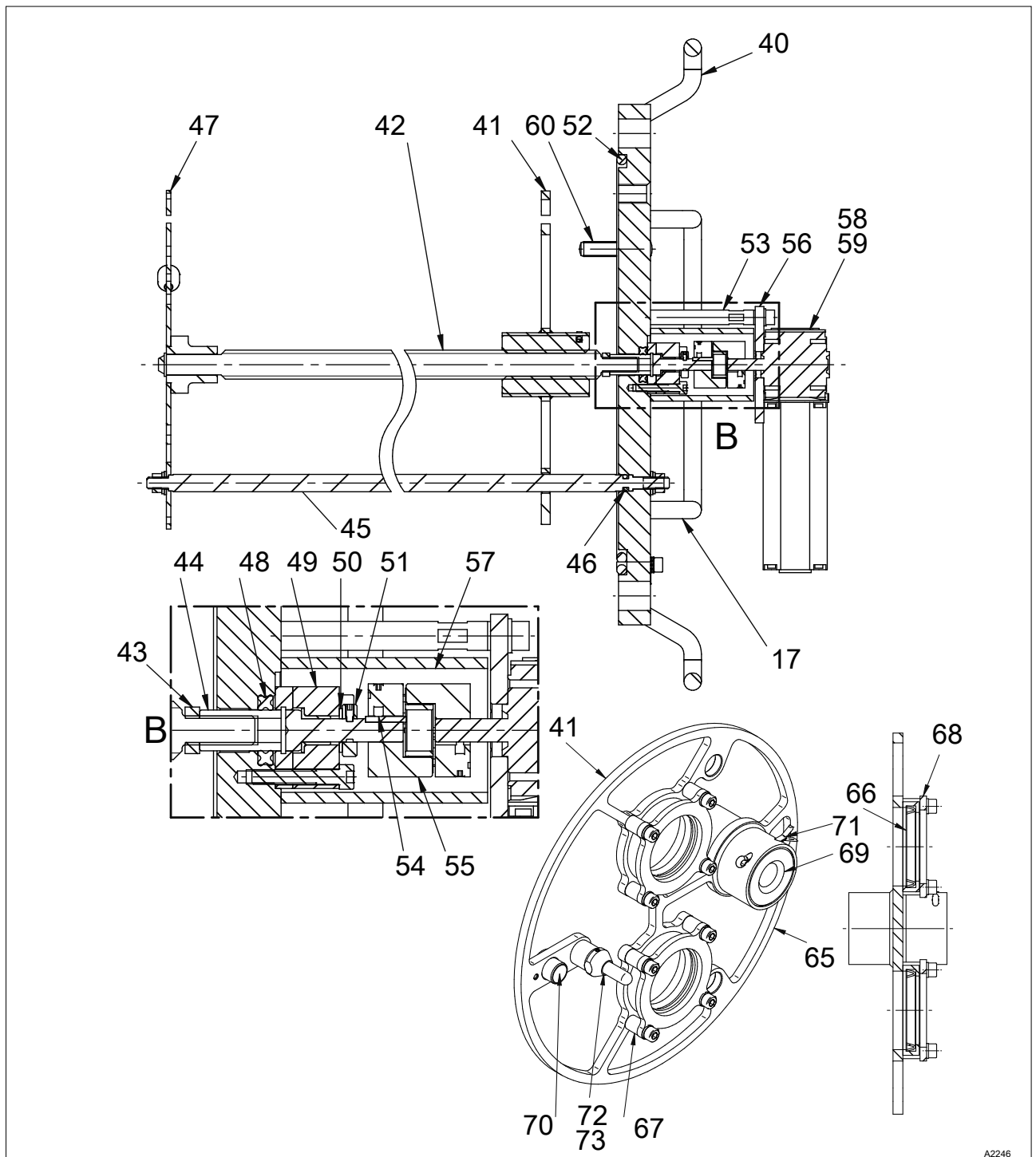
Fig. 62: Spare part diagram, 2 ... 4x350 W, multiple lamp system with wiper
