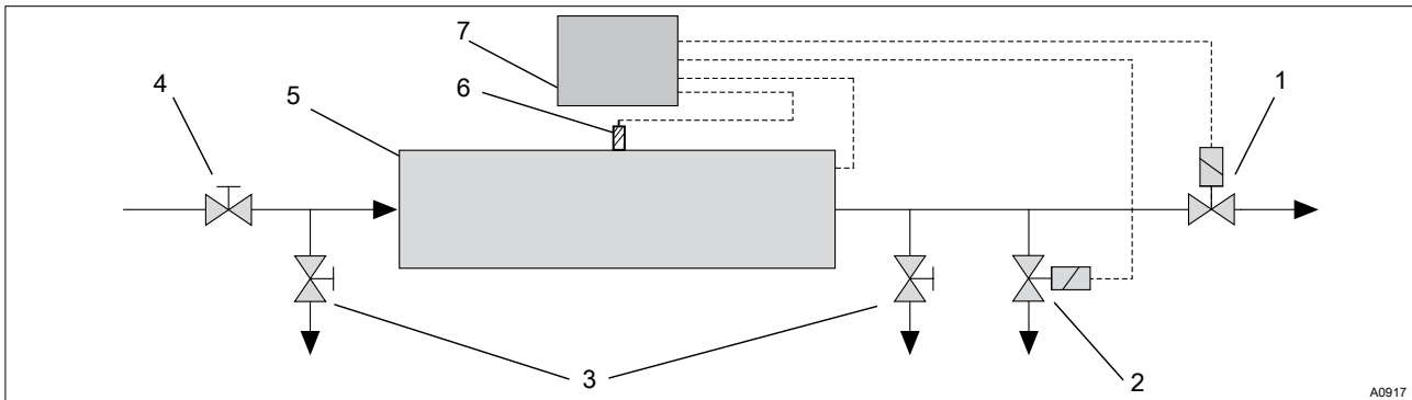
Fig. 1: Typical installation diagram for a UV system
