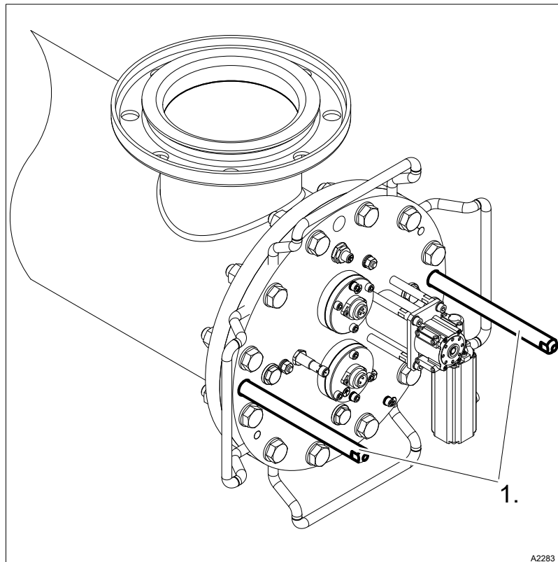
Fig. 9: Assembly aids (1.) 2 units.
