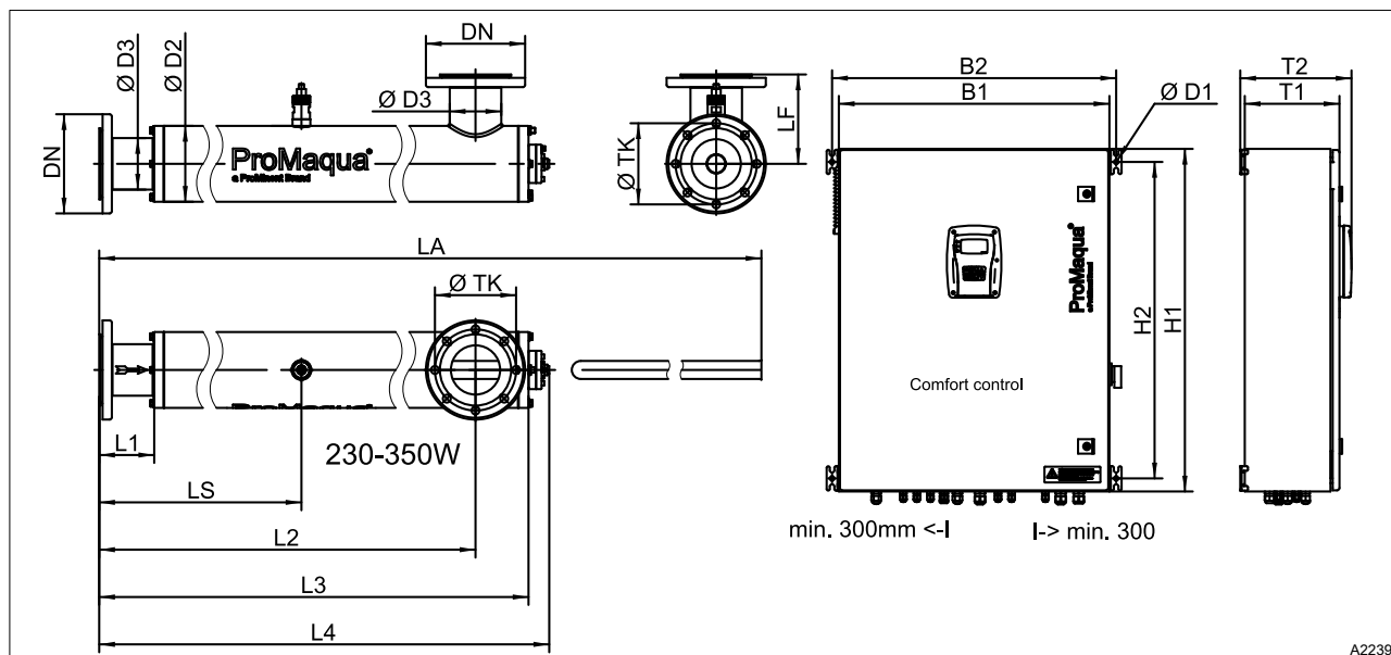
Fig. 48: Dimensional drawing Dulcodes LP 1x230W ... 6x350W.
