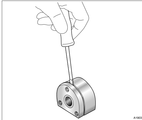
Fig. 33: Bearing cover
