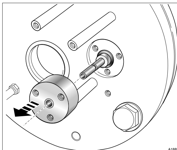
Fig. 19: Bearing cover
