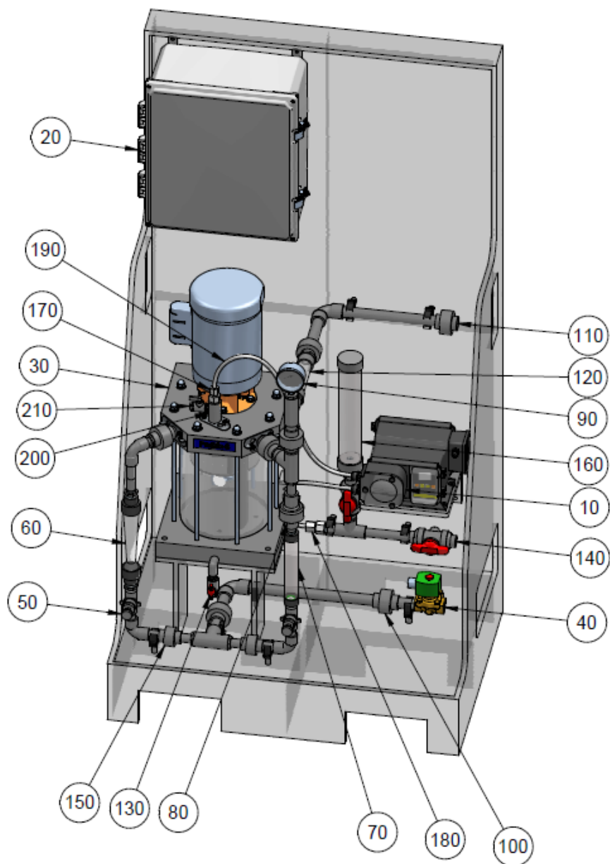
ProMix S TA with Peristaltic Tubing Pump
