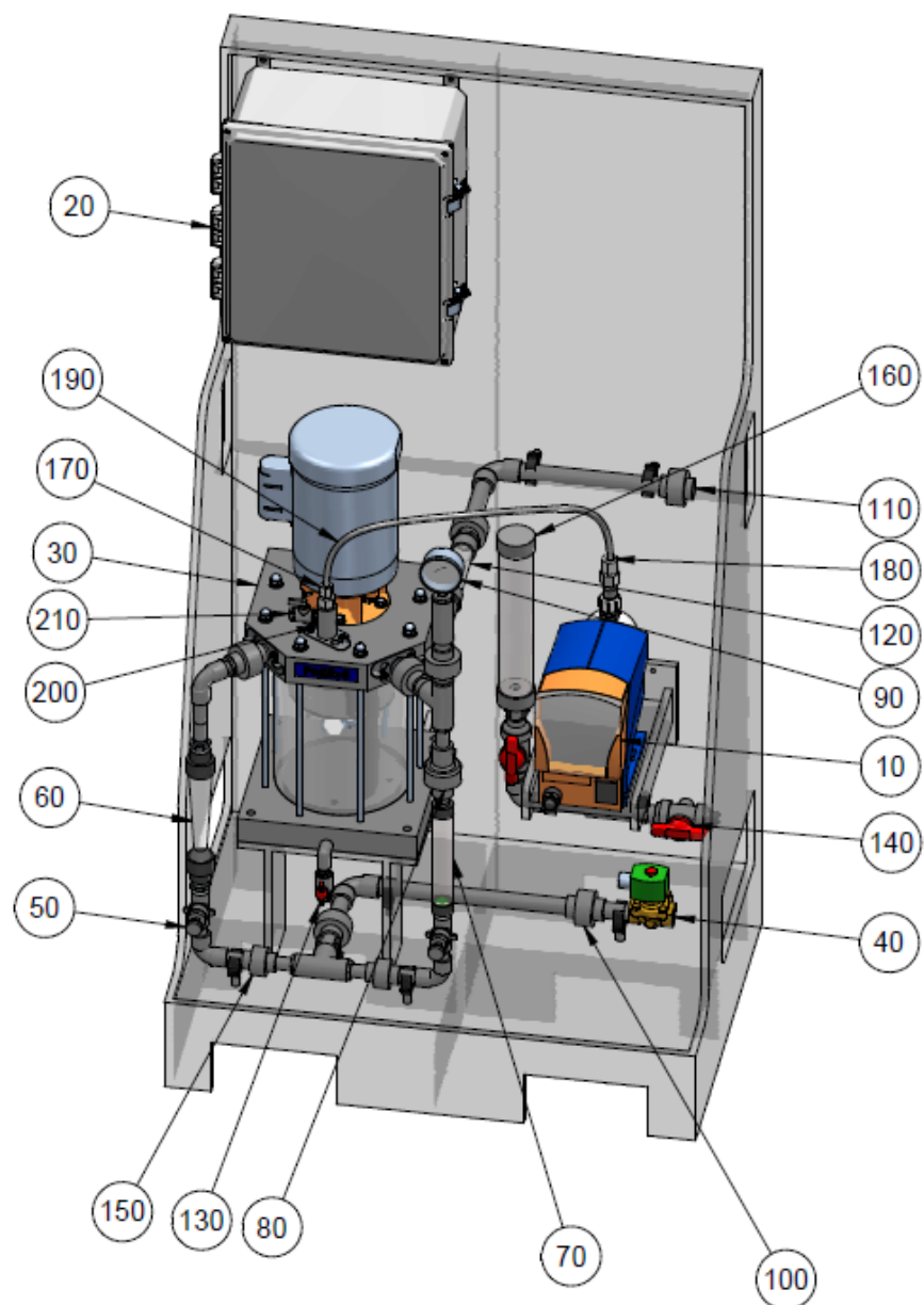
ProMix S DA with Diaphragm Pump
