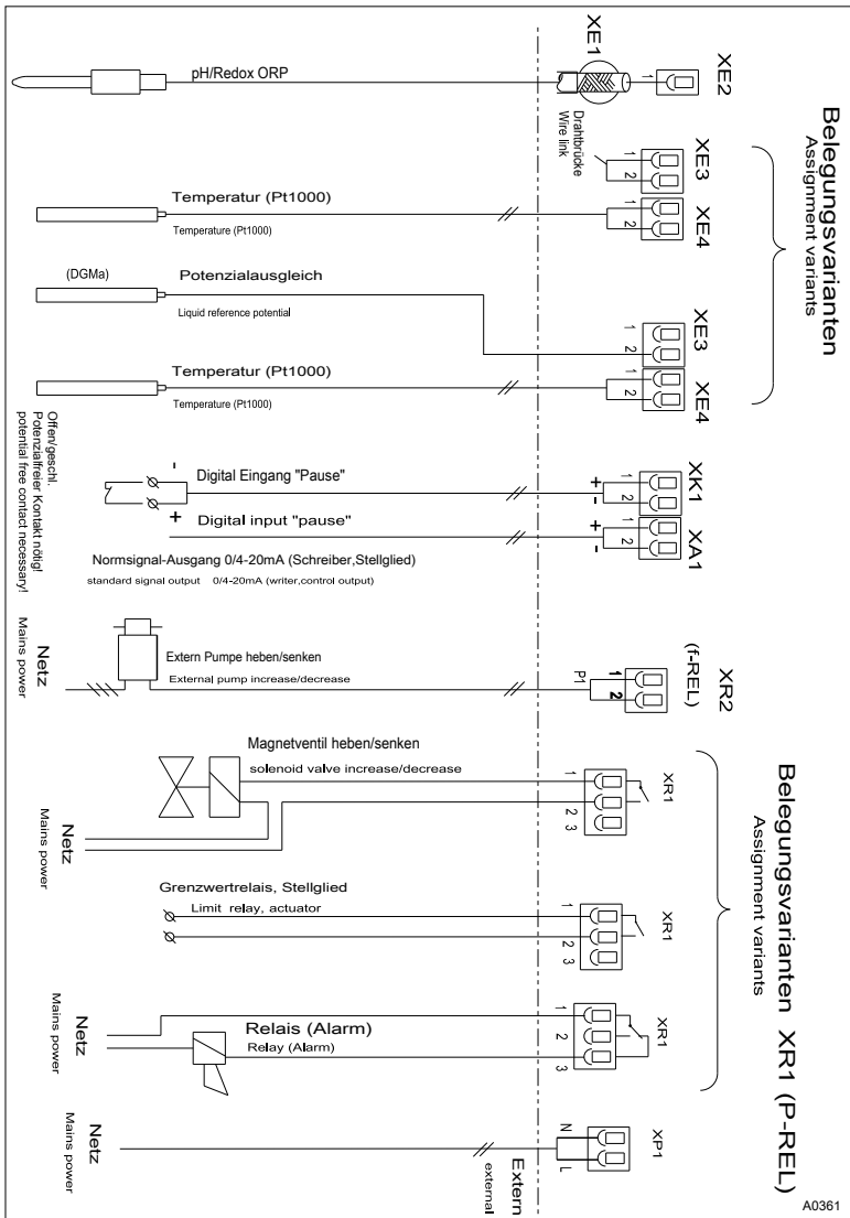
Fig. 15: Terminal diagram
