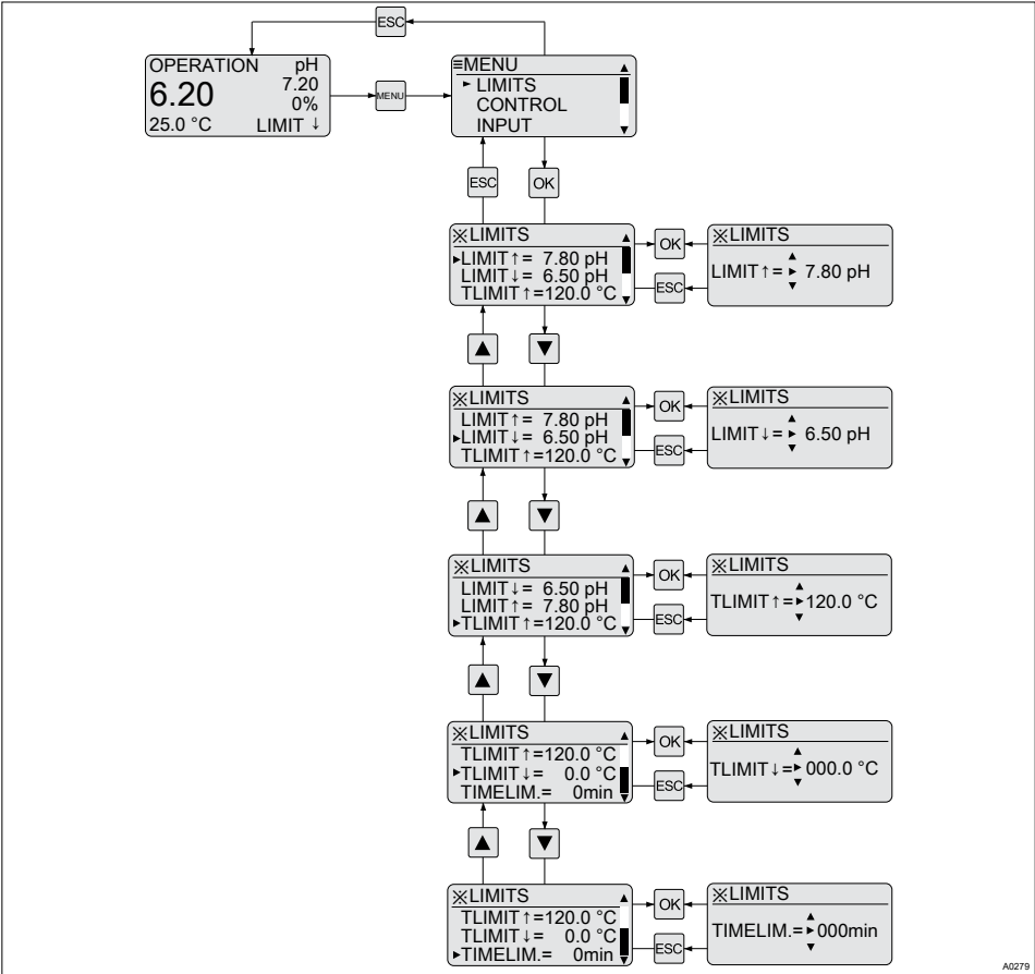
Fig. 28: Limit value setting (LIMITS)
