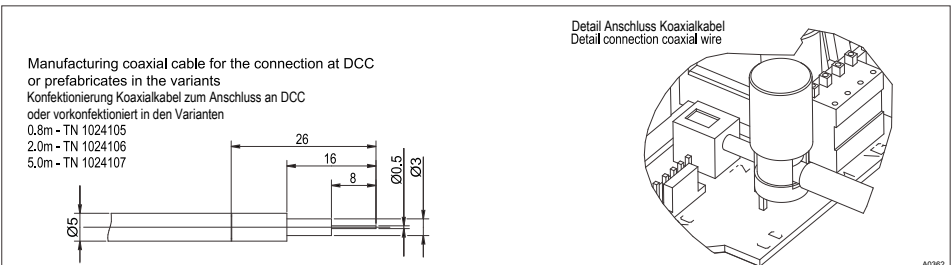
Fig. 13: Installation of Coaxial Cable to Guard Terminal XE1
