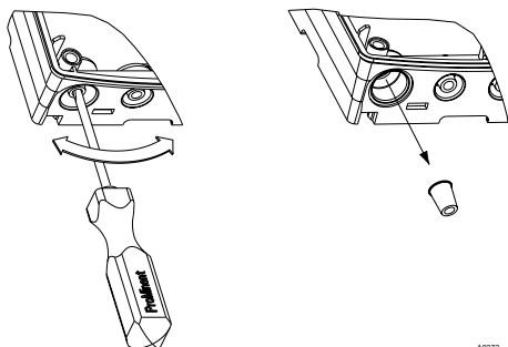
Fig. 16: Punch out threaded holes
