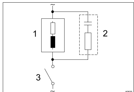
Fig. 18: RC protective circuit for the relay contacts
