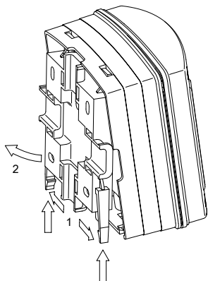
Fig. 3: Removing the wall/pipe bracket
