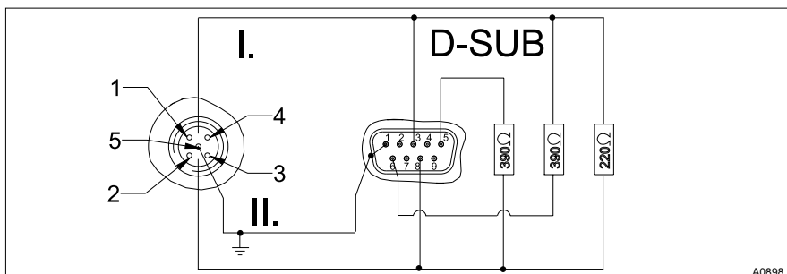
Fig. 6: Connection diagram
