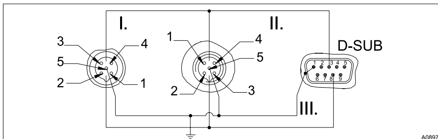
Fig. 5: Connection diagram
