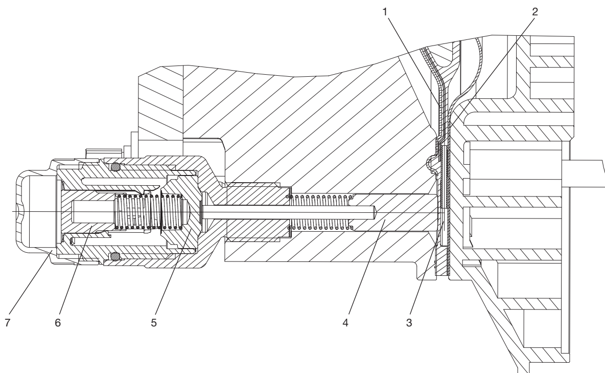
Fig. 12: Section through the diaphragm rupture signalling Sigma (without electrical component parts)
