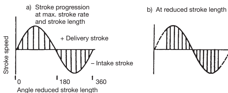
Fig. 6 S3Ba/S3Ca-006-GB
