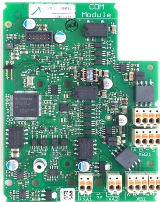
Industrial Communication Driver Card "Com Module"
