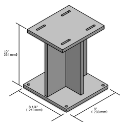
10" PP floor mounting bracket
