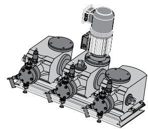
Hydro triplex pump
