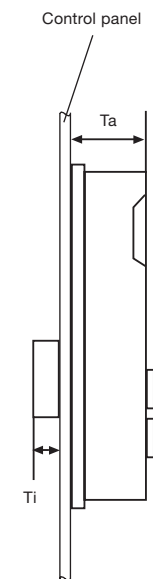
DMT-Dimensions
