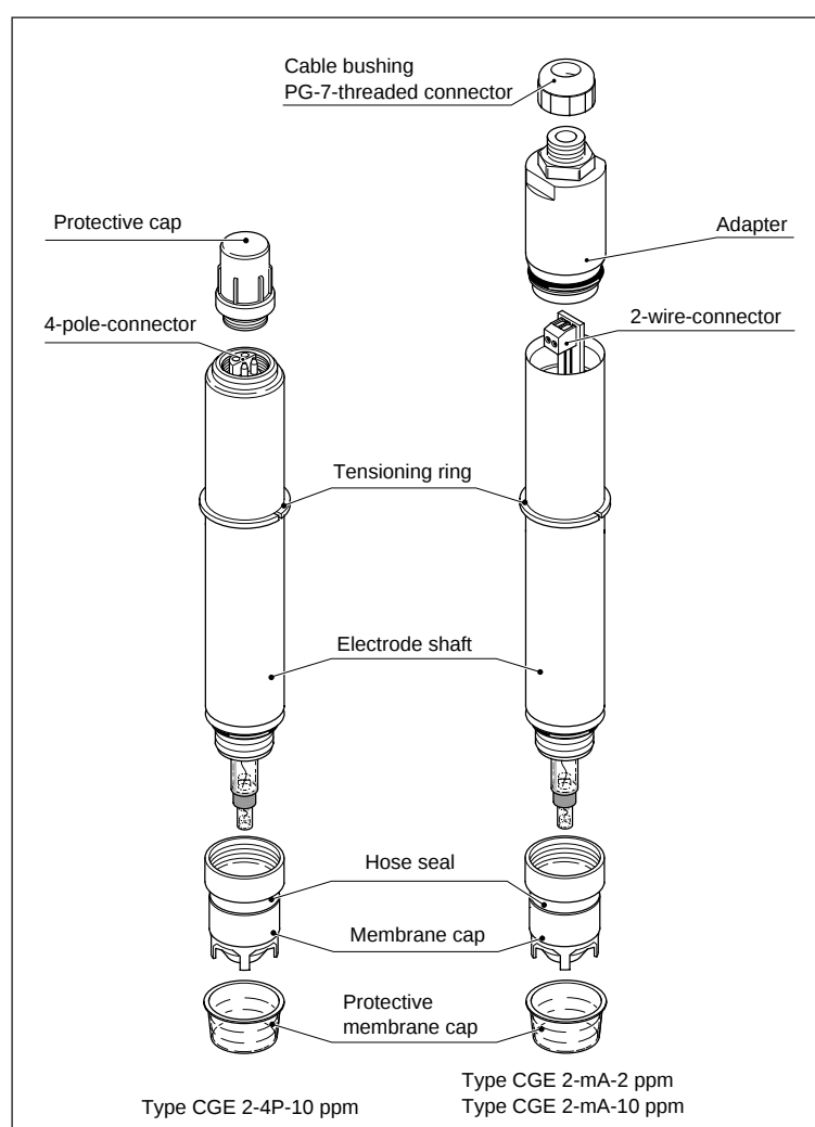
Fig. 2 Sensor designs
