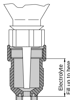
Figure 2: Membran cap
