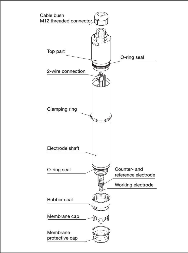
Fig. 1 Sensor designs
