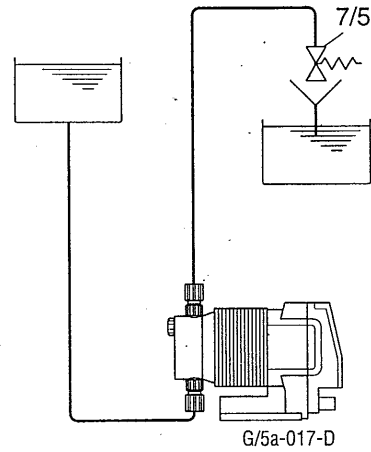
4a) Installation to safely prevent siphoning of hazardous media
