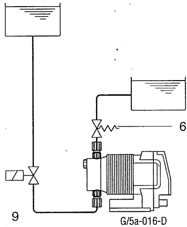
4b) Installation to safely prevent siphoning of hazardous media
