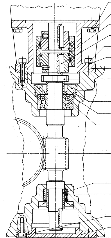
Anbauantrieb Addit driving unit
